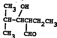
Aldol (IX)
