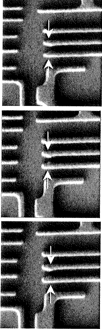
Focus: -0.05μm Focus: 0μm Focus: +0.05μm
