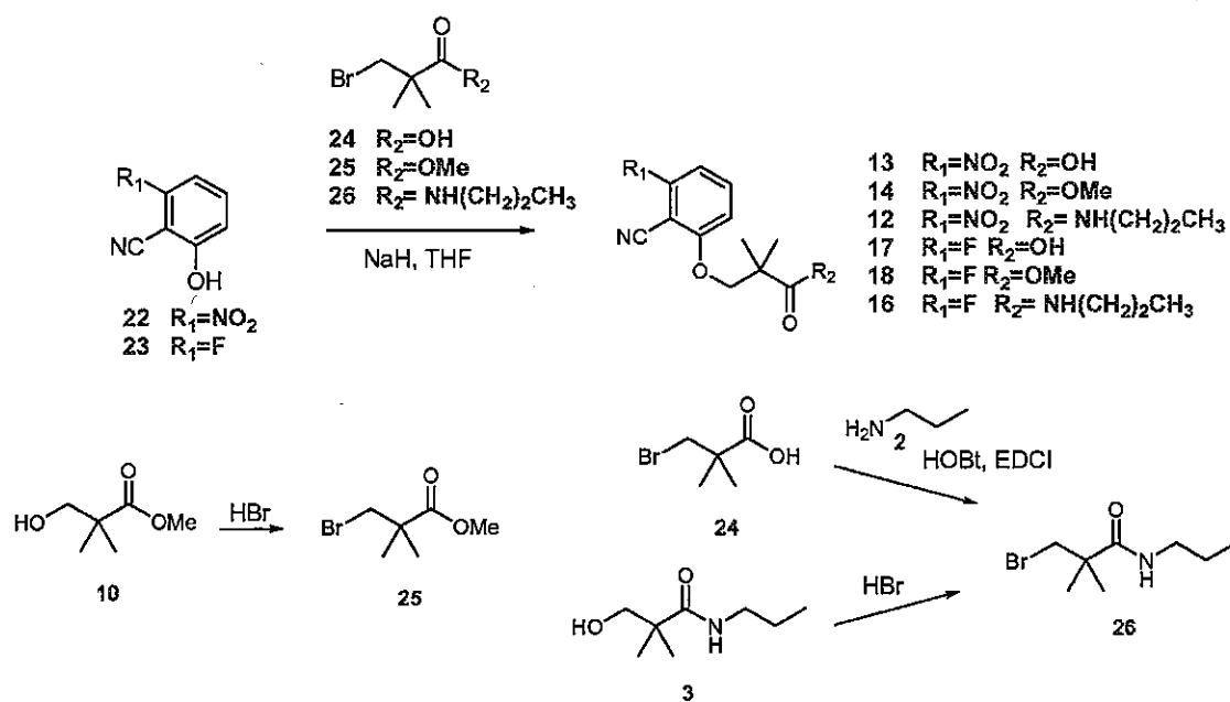
Scheme 10
