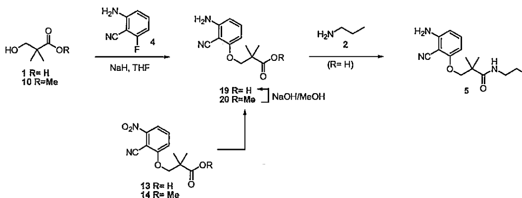
Scheme 8
