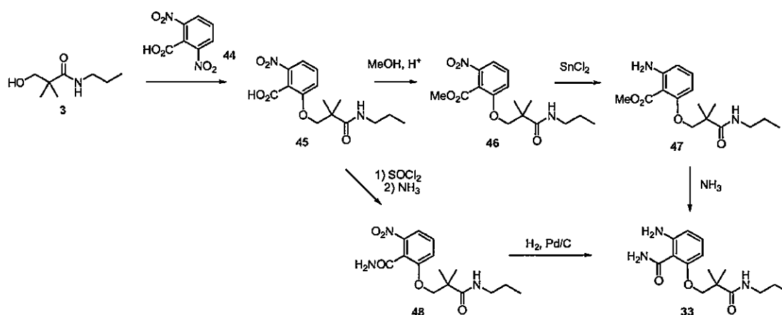
Scheme 16
