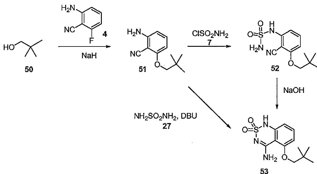
Scheme 17
