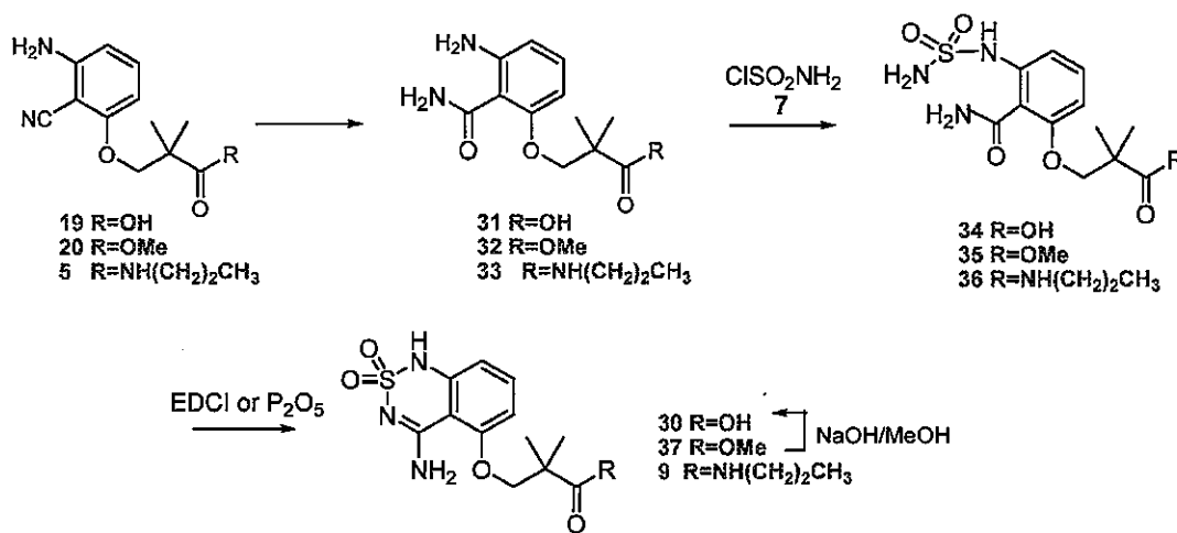
Scheme 14
