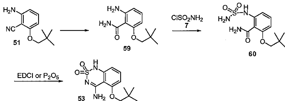
Scheme 21
