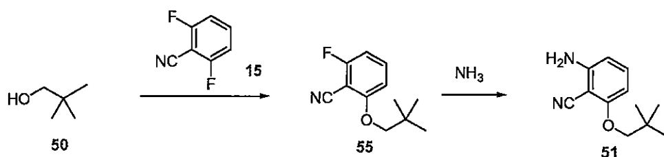
Scheme 19
