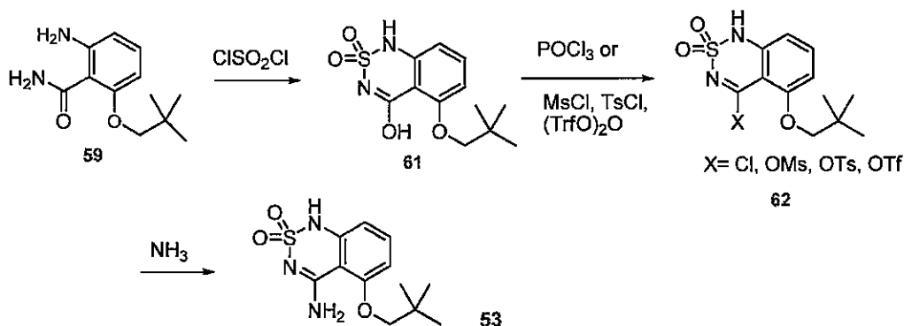
Scheme 22
