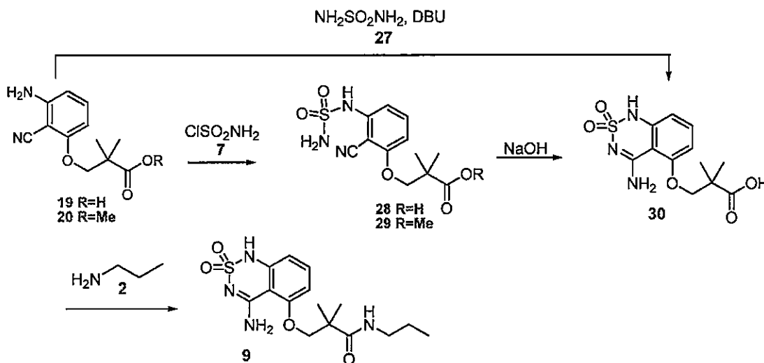
Scheme 13
