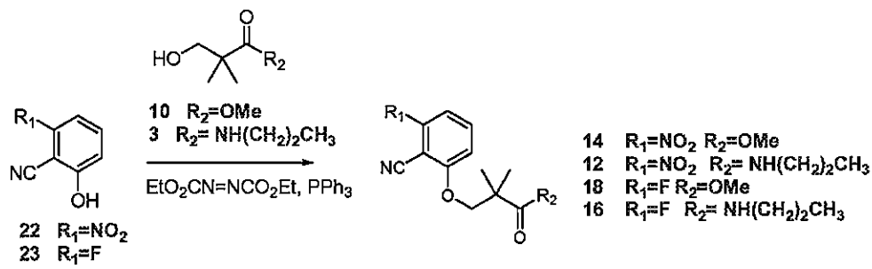
Scheme 11
