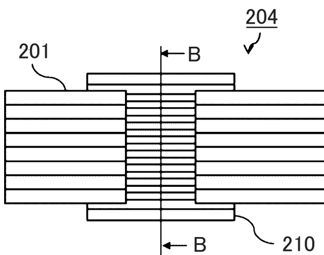
ENLARGED VIEW OF A
