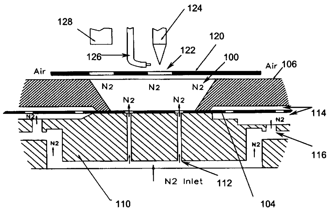
Fig. 3 (Prior Art)
