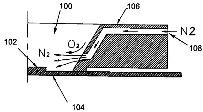
Fig. 1 (Prior Art)
