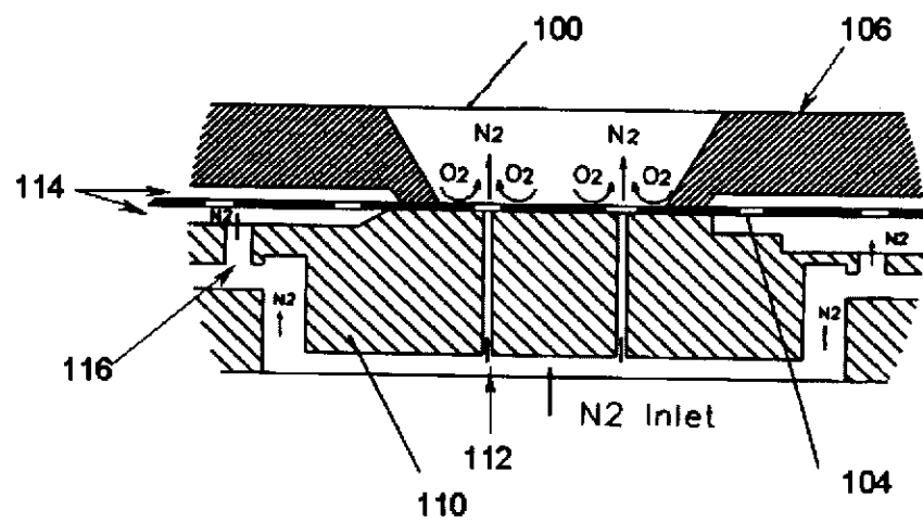
Fig. 2 (Prior Art)
