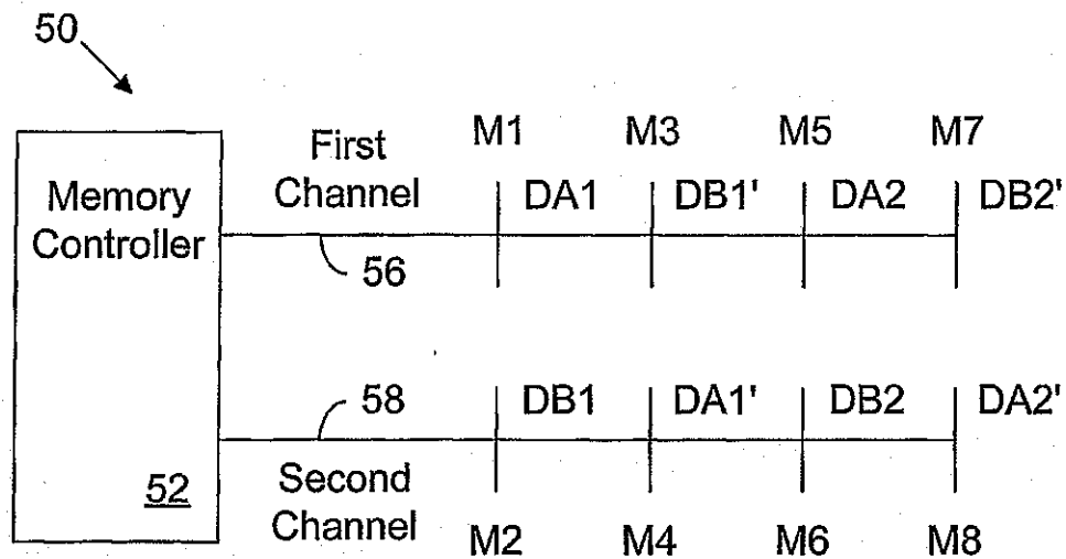
FIG. 1 (Prior Art)
