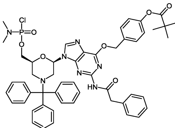
Compound (E1)
