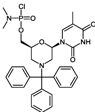
Compound (F1)
