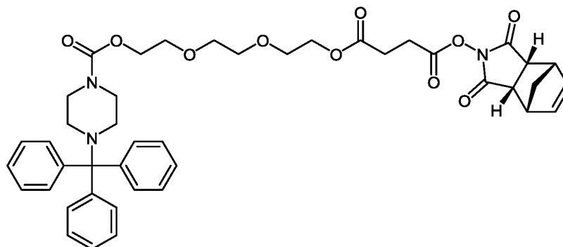
Compound (B)
