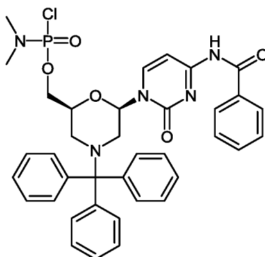
(C1).
