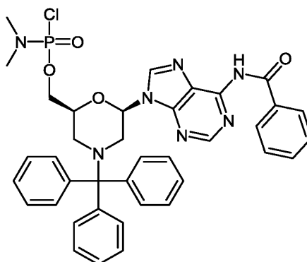
Compound (D1)
