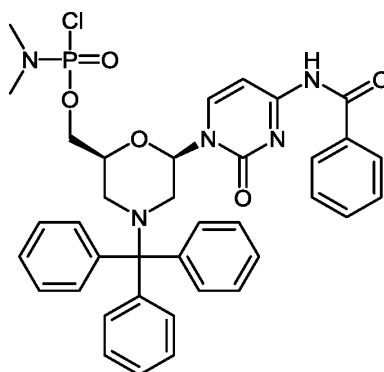
Compound (C1)
