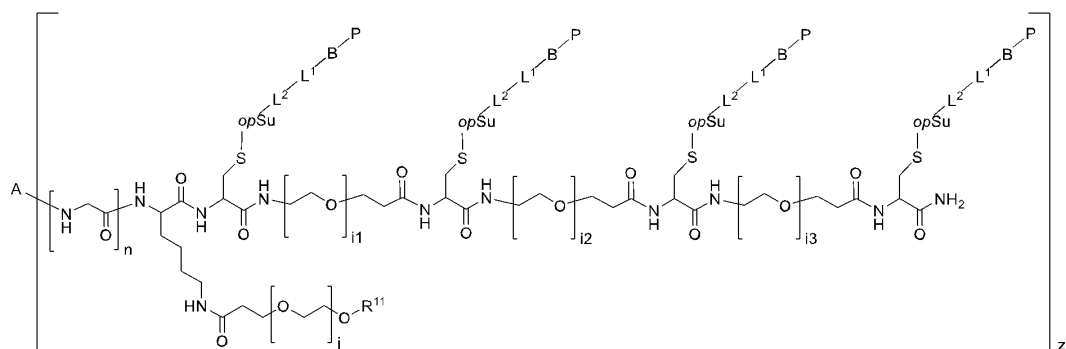
(conjugate III-a-1-4)
