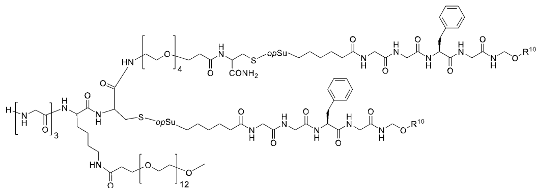
(I-a-1-2-4)
