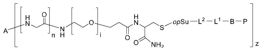
(conjugate III-a-0-2)
