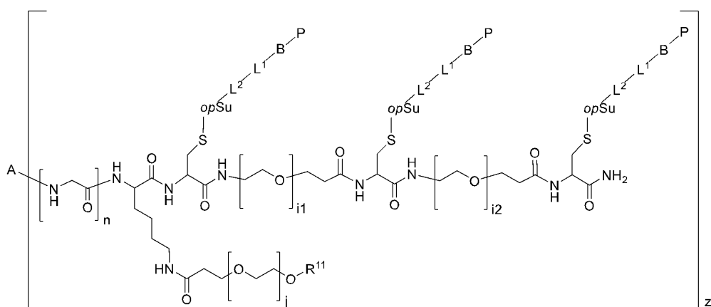
(conjugate III-a-1-3)
