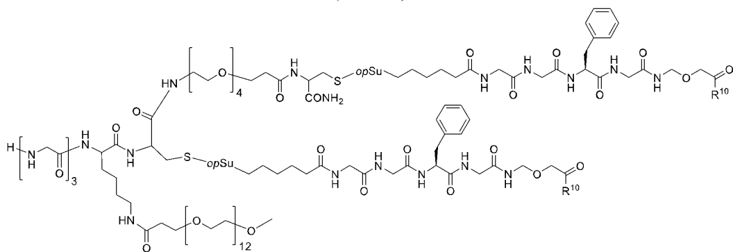
(I-a-1-2-6).
