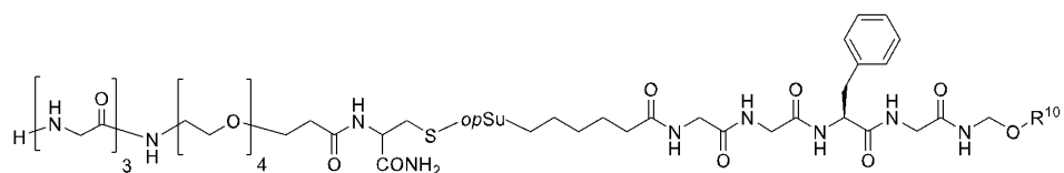
(I-a-0-2-1)
