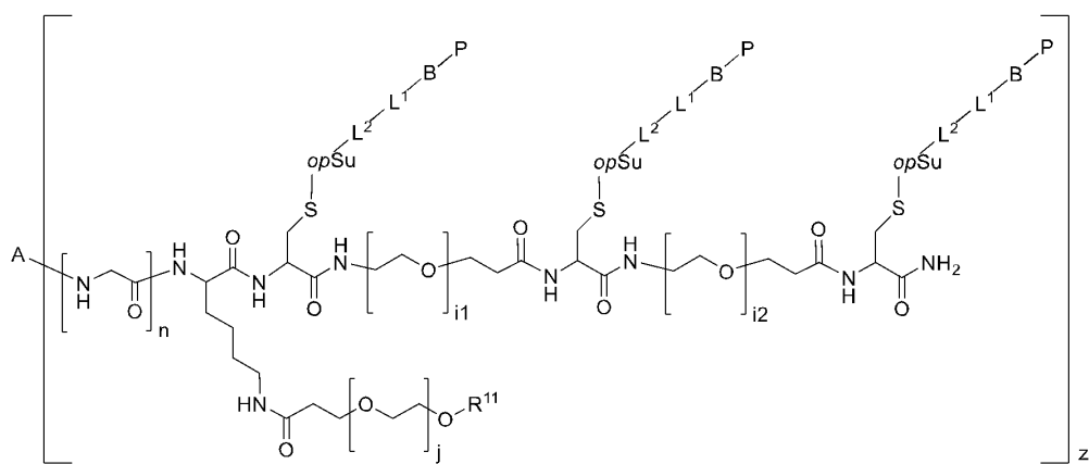
(conjugate III-a-1-3)
