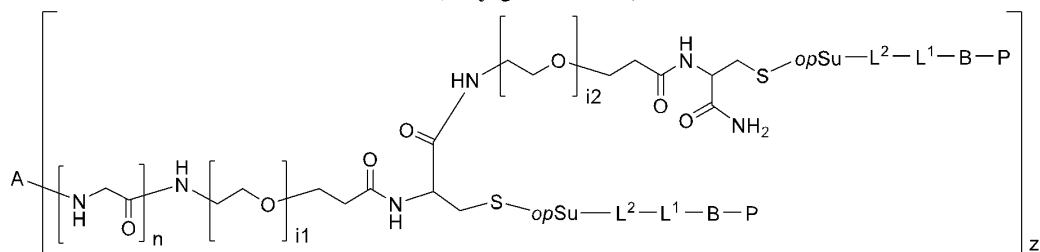
(conjugate III-a-0-3)
