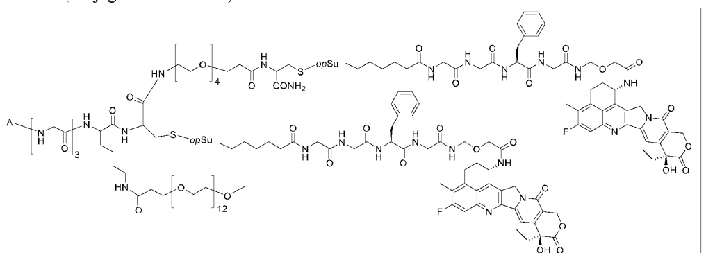
(conjugate III-a-1-2-4-1)
