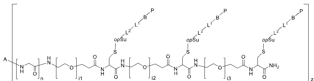
(conjugate III-a-0-4)
