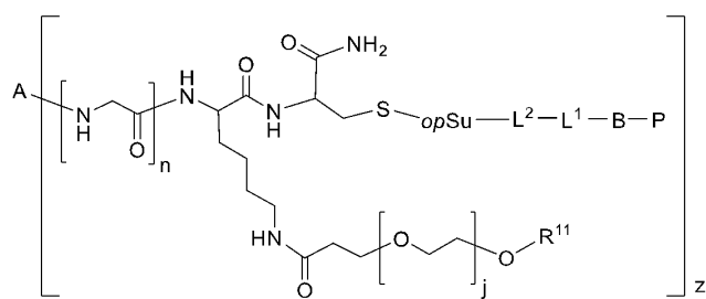
(conjugate III-a-1-1)
