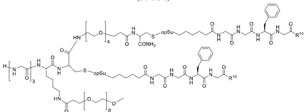
(I-a-1-2-2)
