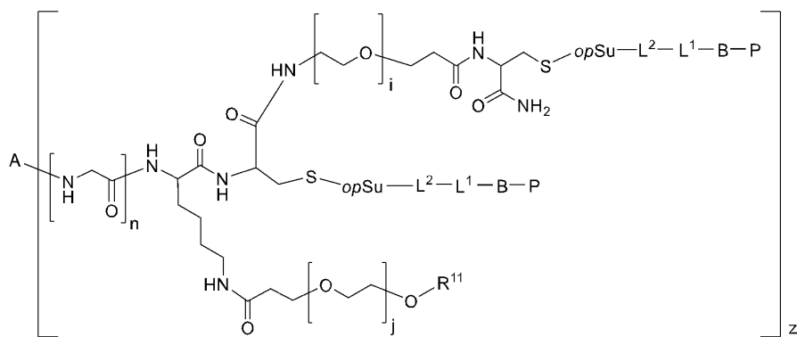
(conjugate III-a-1-2)
