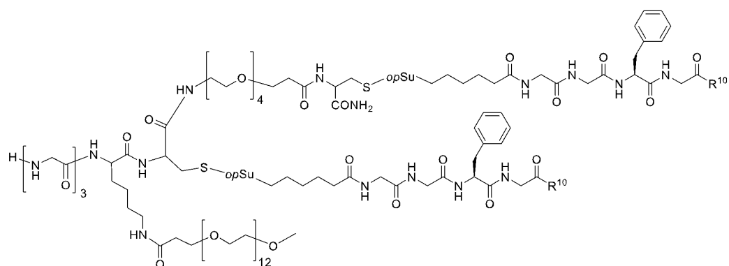
(I-a-1-2-5)
