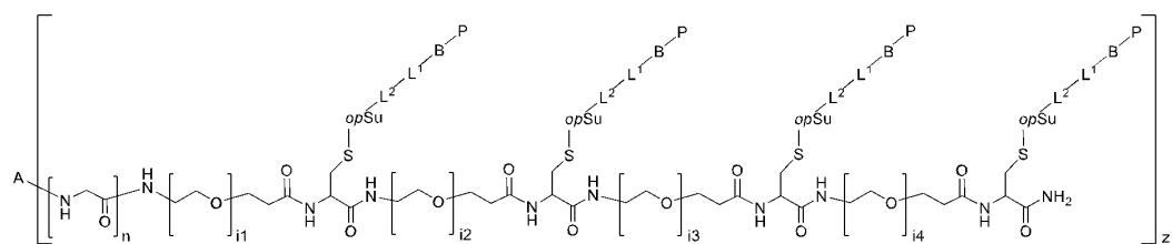
(conjugate III-a-0-5)
