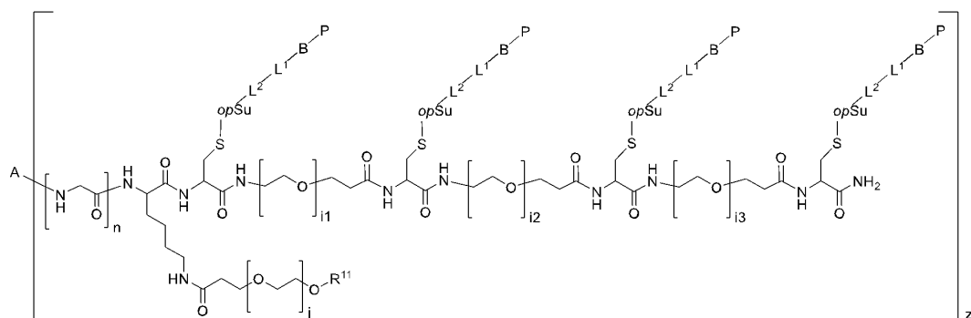
(conjugate III-a-1-4)
