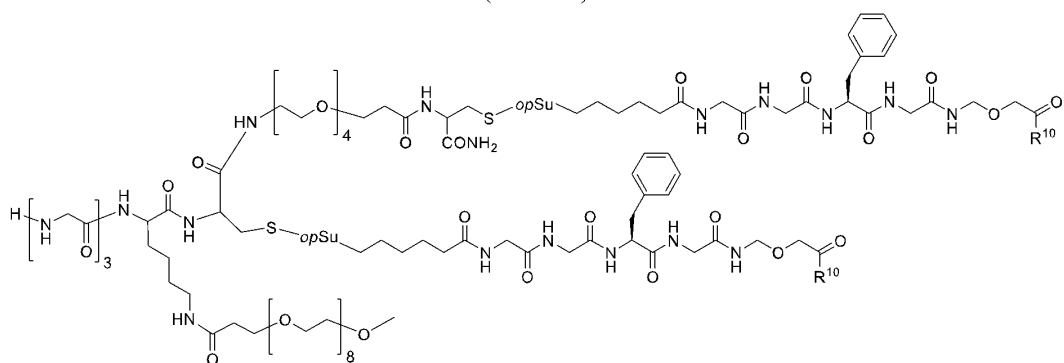
(I-a-1-2-3).
