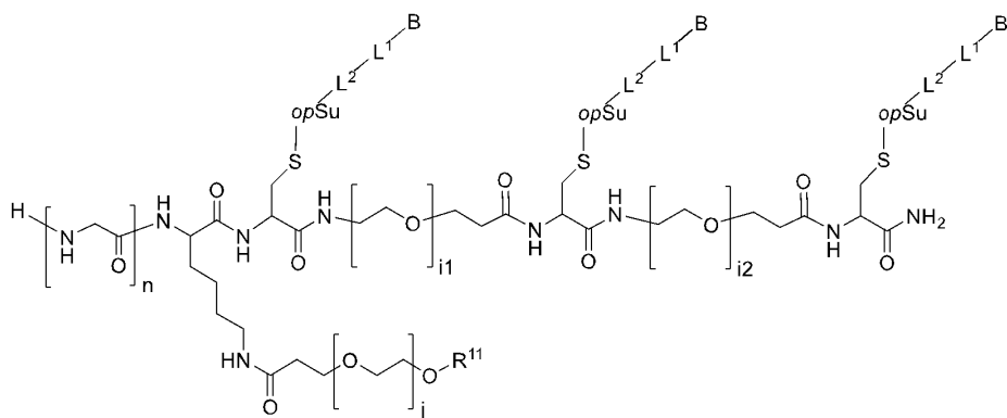
(I-a-1-3)
