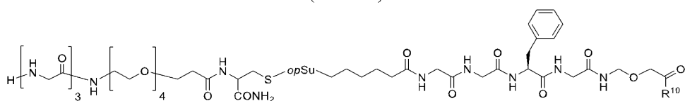
(I-a-0-2-3).
