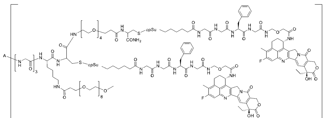
(conjugate III-a-1-2-1)
