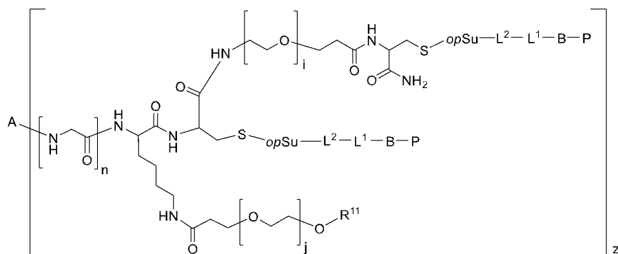
(conjugate III-a-1-2)
