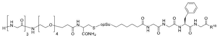
(I-a-0-2-2)
