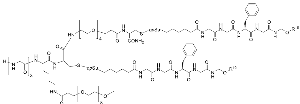
(I-a-1-2-1)
