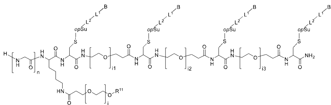
(I-a-1-4).
