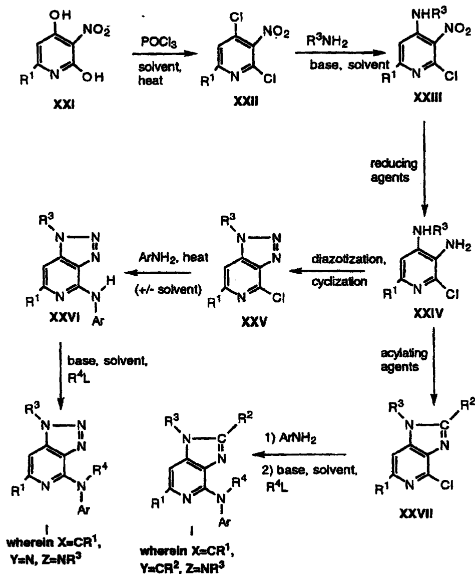
Scheme 7
