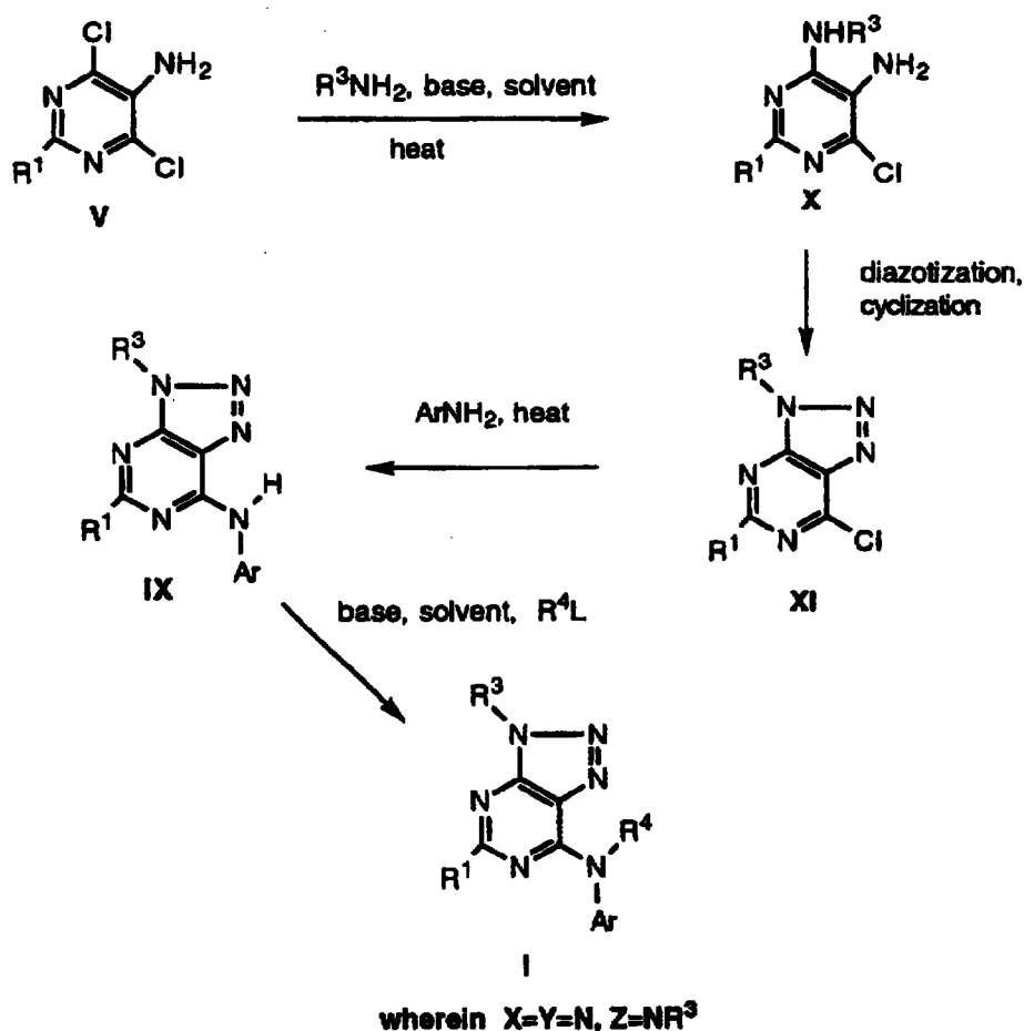
Scheme 2
