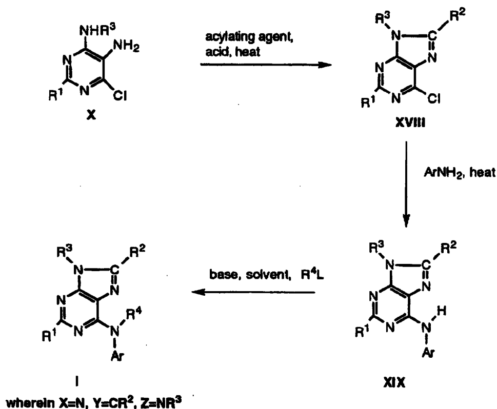
Scheme 5
