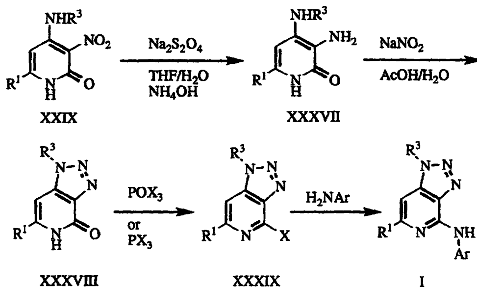
Scheme 11
