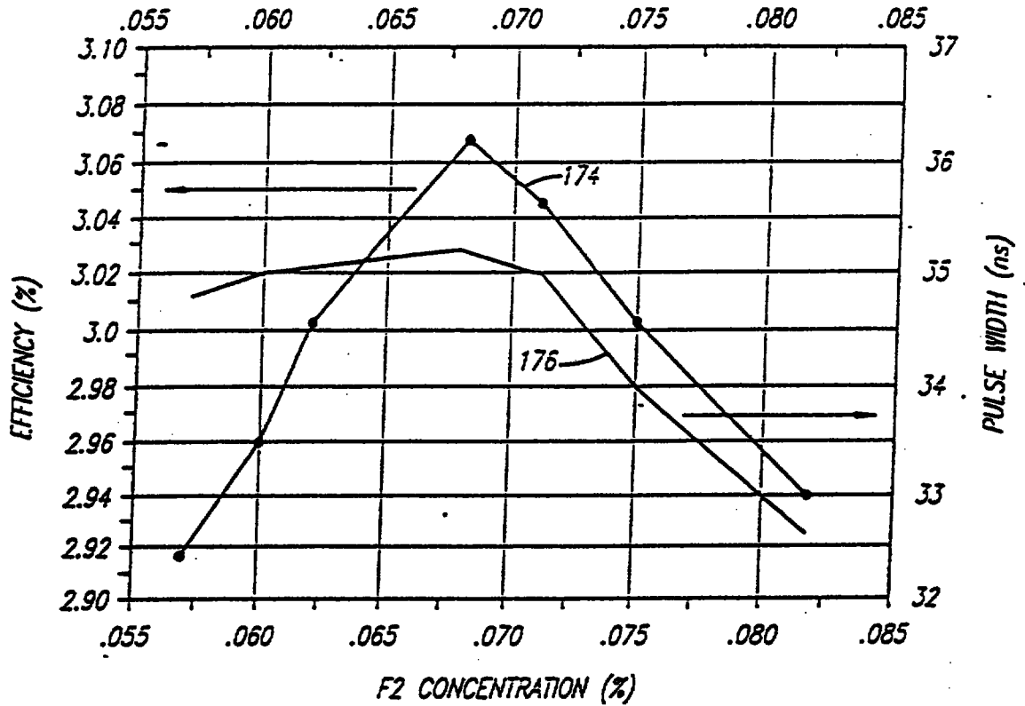
EFFICIENCY & PULSEWIDTH VS. F2 CONCENTRATION
