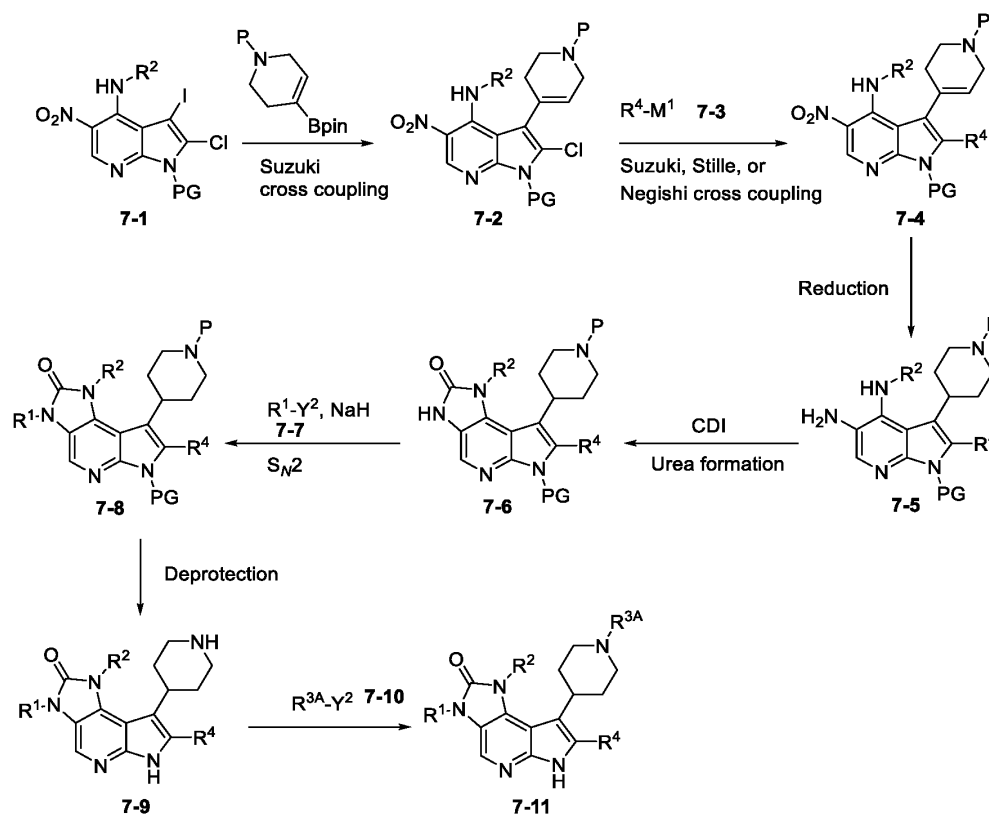
Scheme 7.
