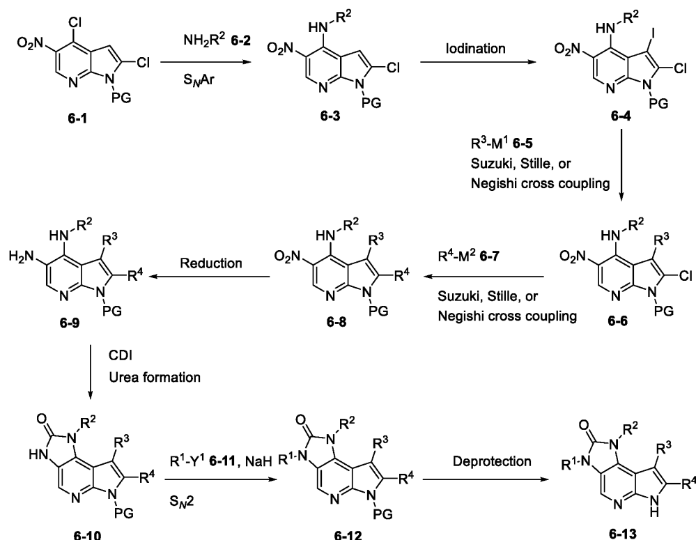
Scheme 6.
