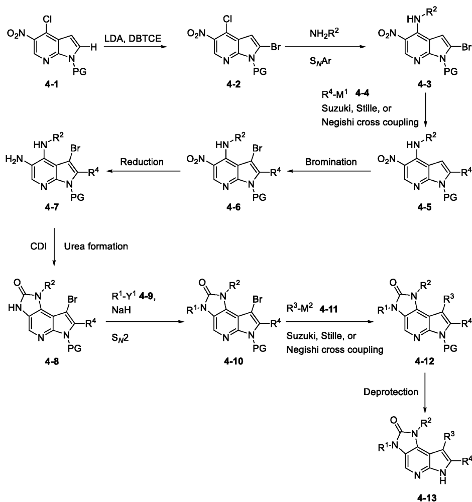
Scheme 4.
