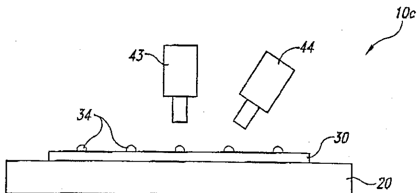
Fig. 1C (Prior Art)
