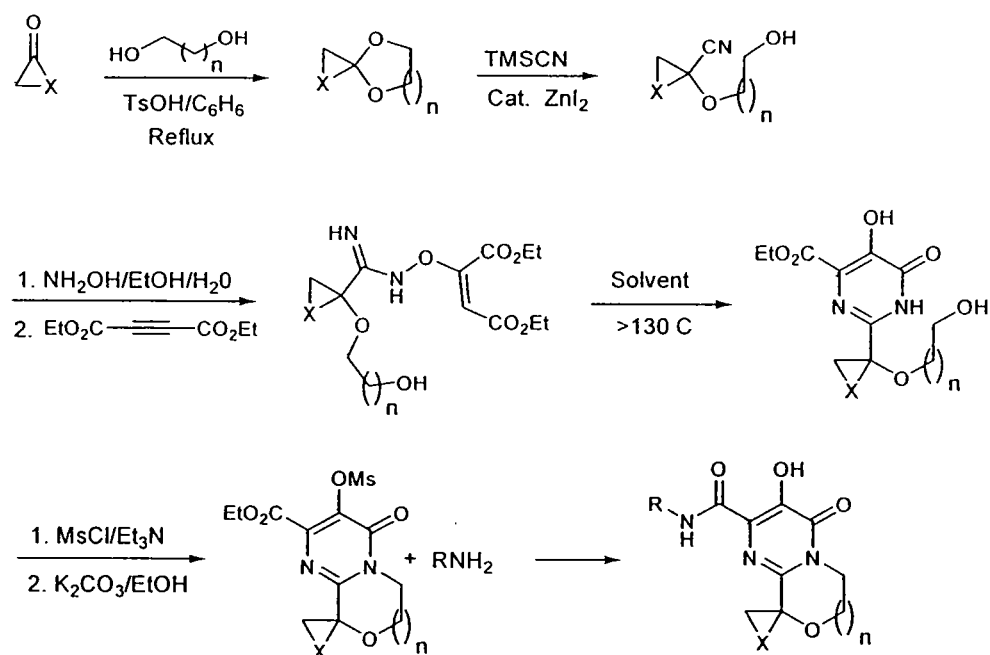
5 Scheme 2.
