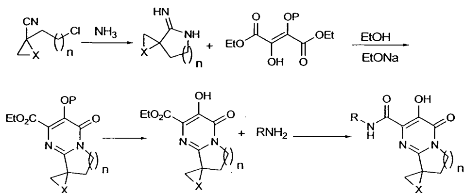
5 Scheme 4.
