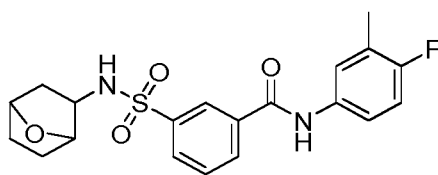
Compound 128
