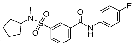
Compound 46
