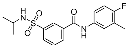
Compound 73
