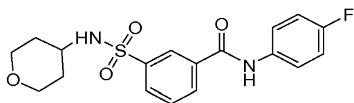
35 Compound 1
