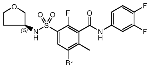
Compound 187
