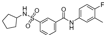
Compound 11
