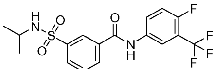
Compound 74
