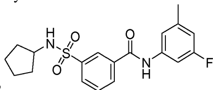
Compound 12
