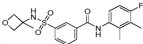
Compound 115
