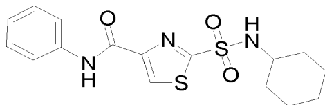
Compound 64
