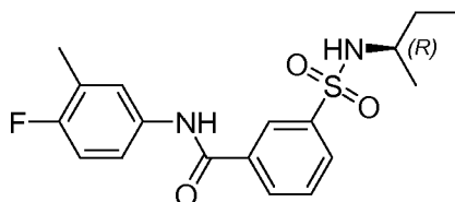
Compound 98
