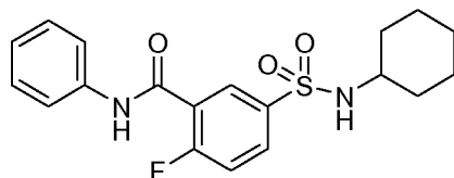
Compound 19
