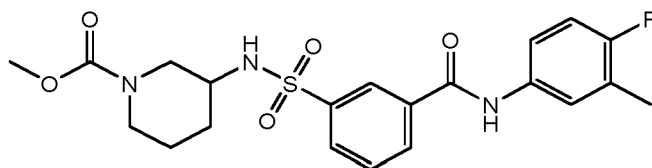
Compound 159
