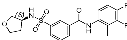
Compound 118
