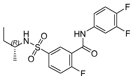
Compound 100
