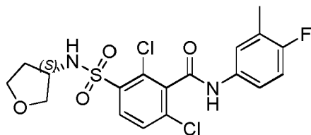
Compound 125
