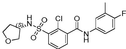
Compound 124
