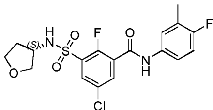
Compound 123
