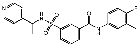
Compound 161
