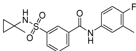
Compound 94
