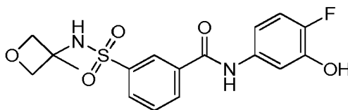
15 Compound 108
