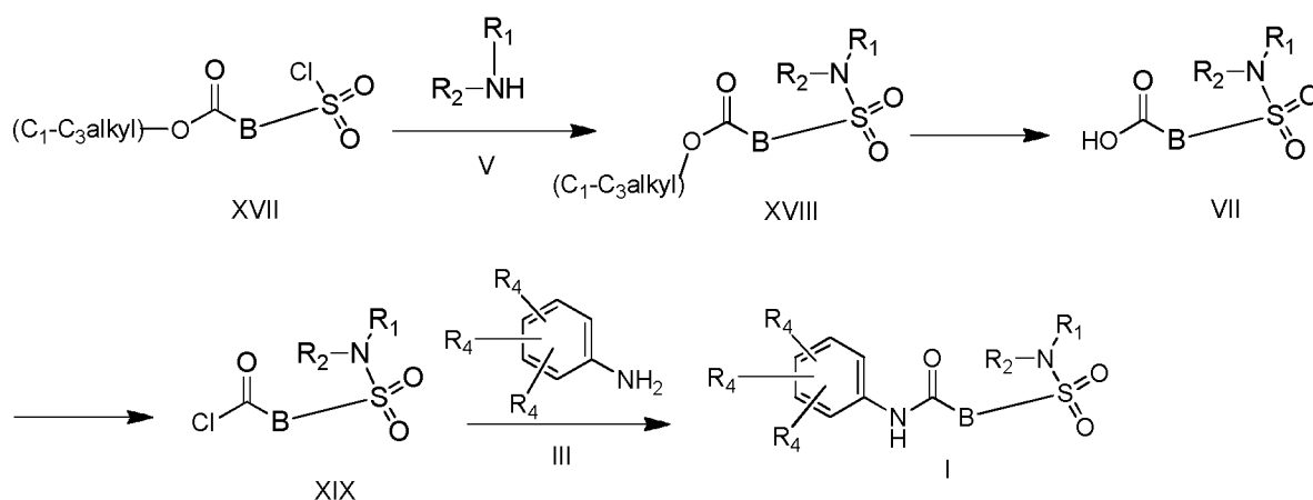
Scheme 6
