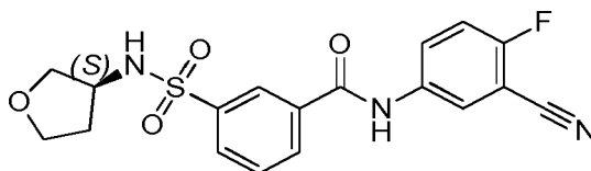
Compound 105
