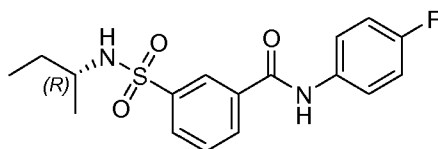
Compound 70
