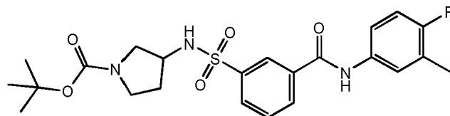
Compound 156
