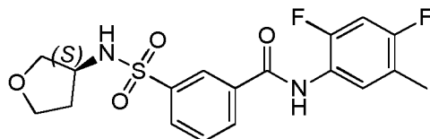
Compound 106
