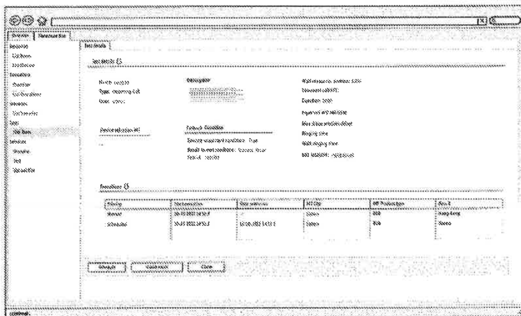
Fig. 18 - Incoming call test details
