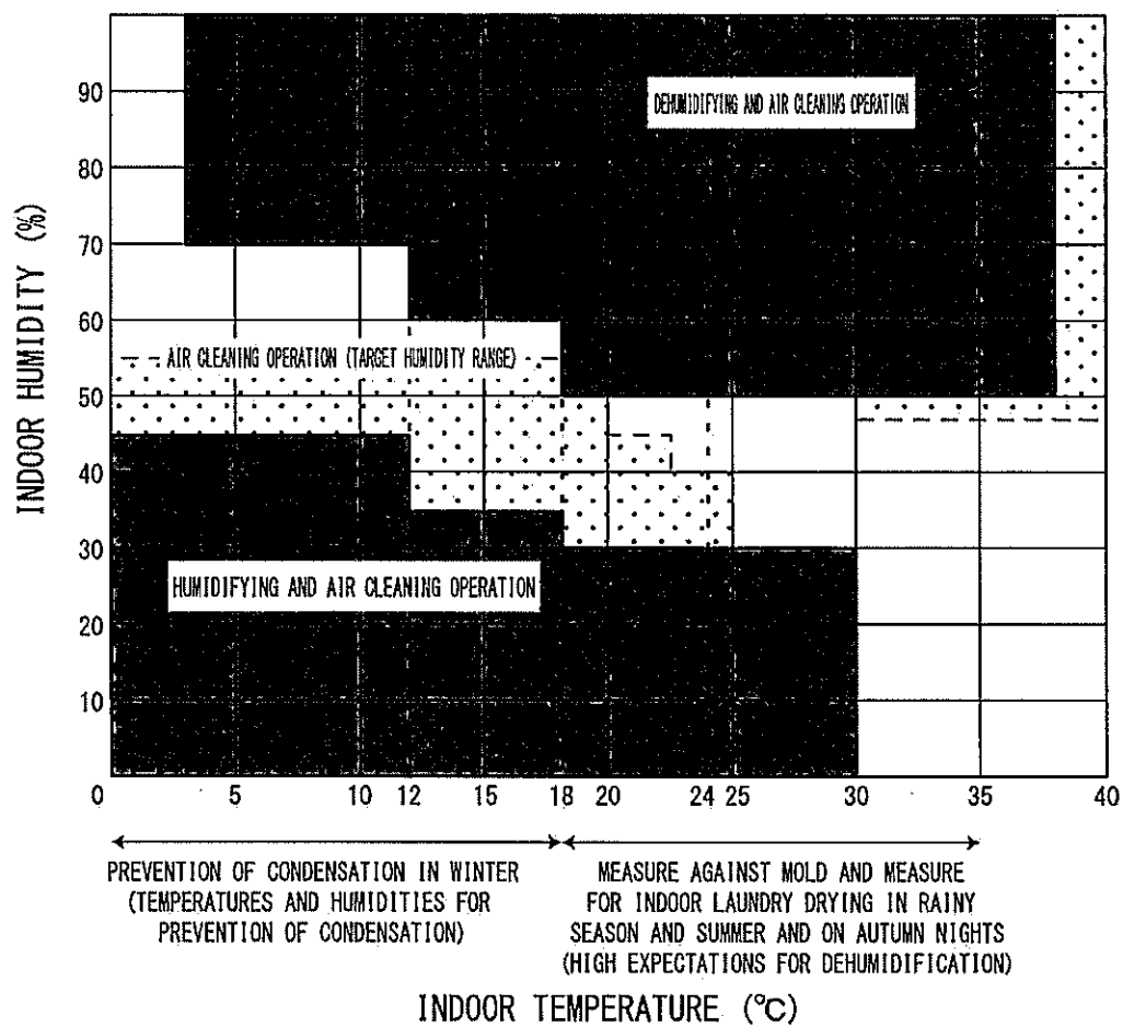
FIG. 8 TABLE (DARK) FOR LIVING ROOM IN DARK STATE
