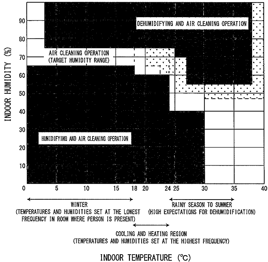
FIG. 11 TABLE (DARK) FOR BEDROOM IN DARK STATE
