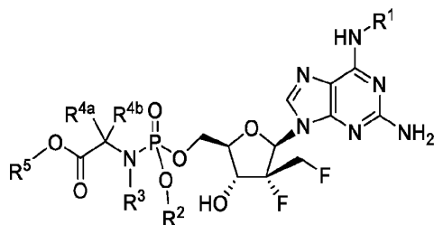
Formula IIIa
