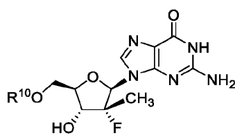
Formula VIII
