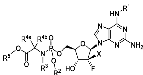
Formula III
