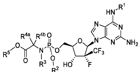
Formula IIIb
