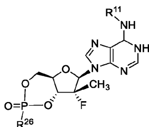
Formula X'
