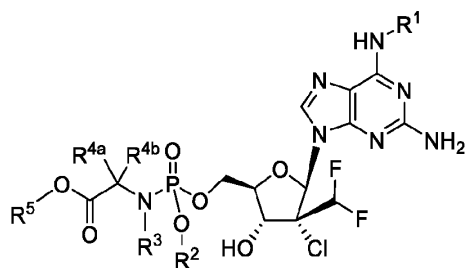
Formula IVc
