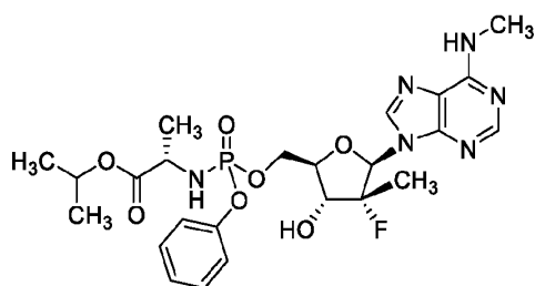
Compound 3
