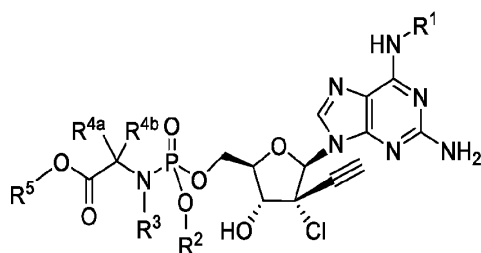
Formula IVe
