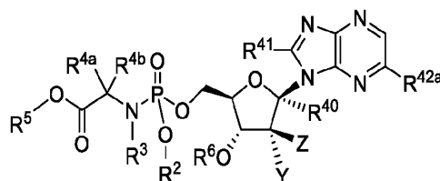
Formula VIIa
