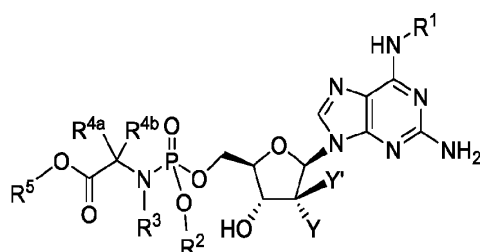
Formula V
