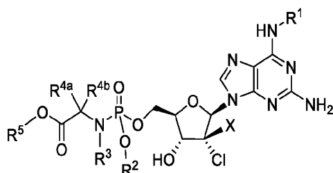
Formula IV
