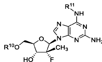
Formula IX
