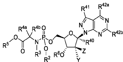
Formula VIIc
