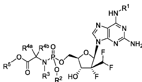
Formula IIIc
