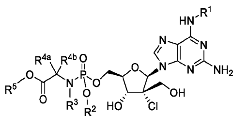
Formula IVf
