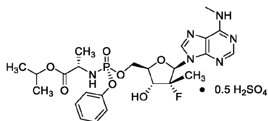
Compound 4B
