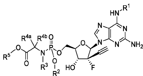
Formula IIIe
