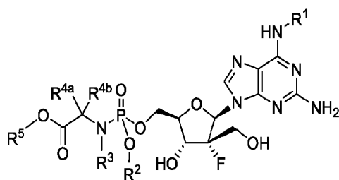
Formula IIIf
