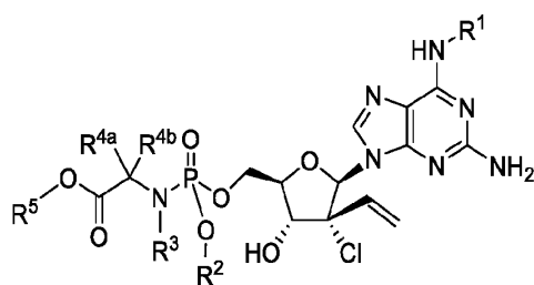
Formula IVd
