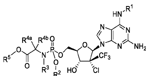
Formula IVb
