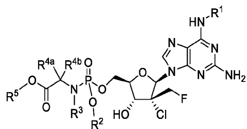
Formula IVa
