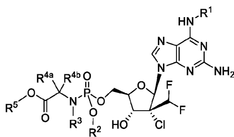
Formula IVc
