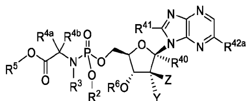
Formula VIIa
