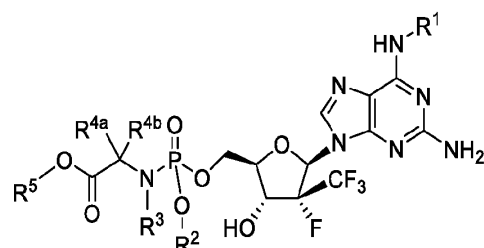
Formula IIIb
