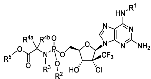
Formula IVb
