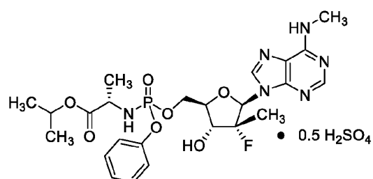
Compound 4
