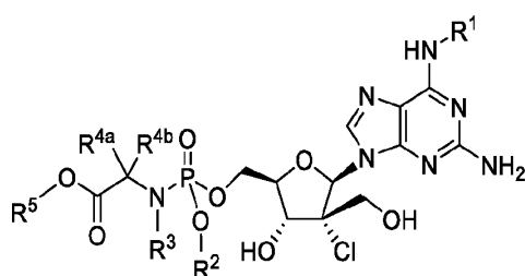
Formula IVf
