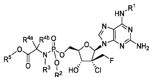
Formula IVa
