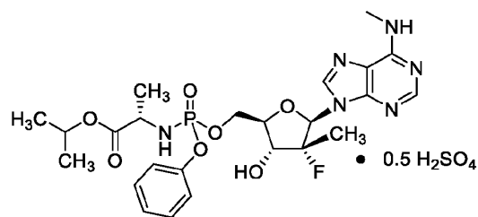
Compound 4
