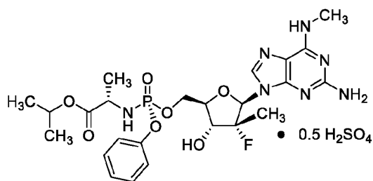
Compound 2B
