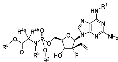
Formula IIId
