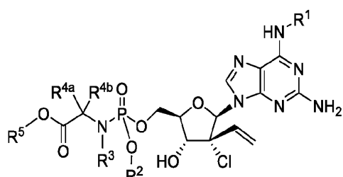
Formula IVd
