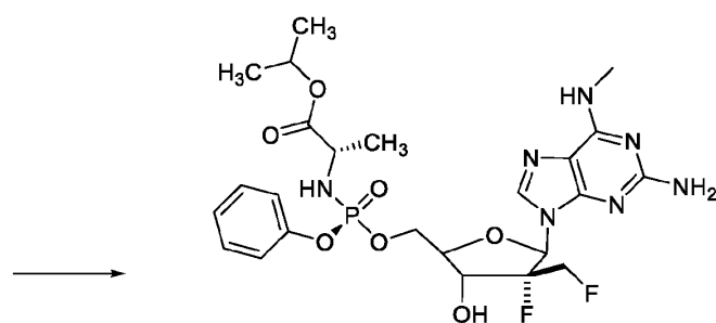
Compound 6
