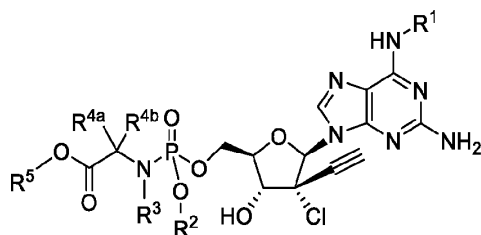
Formula IVe
