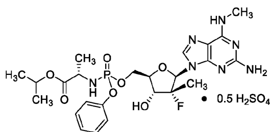
Compound 2
