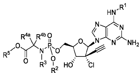
Formula IVe
