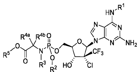
Formula IVb
