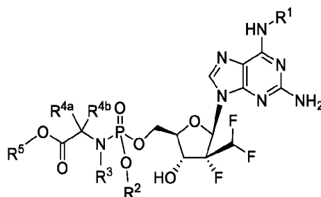
Formula IIIc
