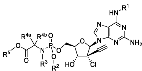
Formula IVe
