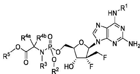
Formula IIIa
