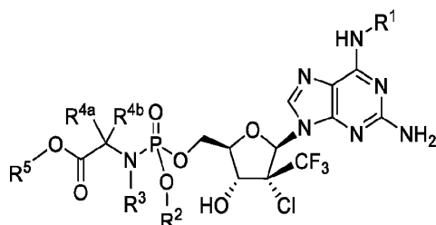
Formula IVb
