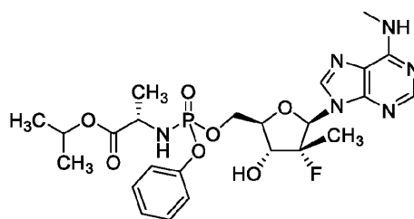
Compound 3
