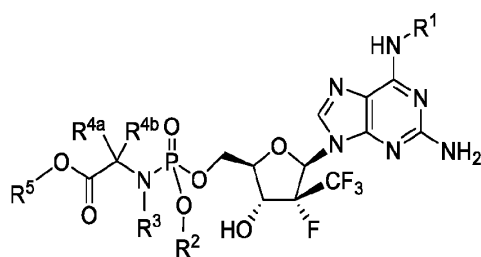
Formula IIIb
