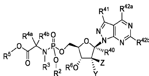
Formula VIIc
