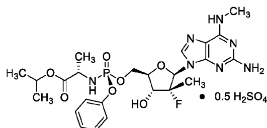
Compound 2A
