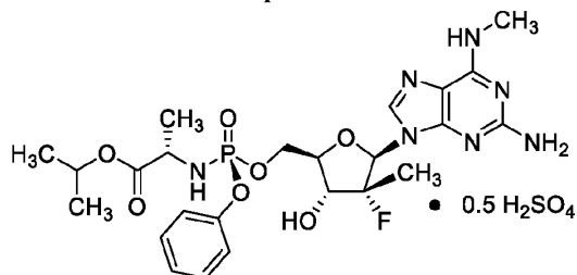
Compound 1B
