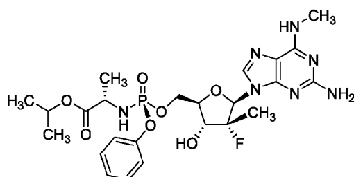
Compound 1A
