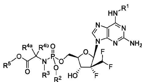
Formula IIIc
