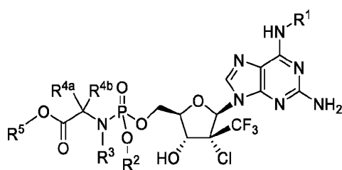
Formula IVb
