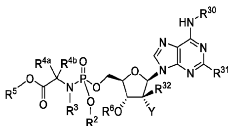
Formula XIII
