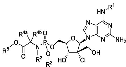
Formula IVf
