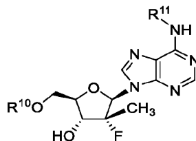
Formula X
