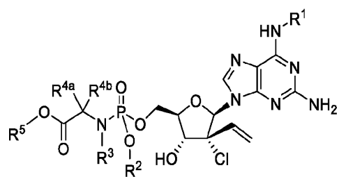
Formula IVd
