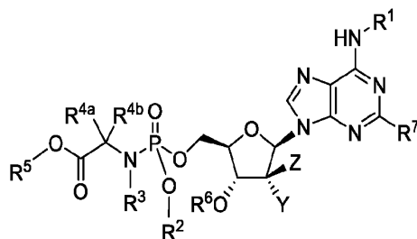
Formula VI
