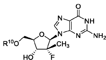
Formula VIII
