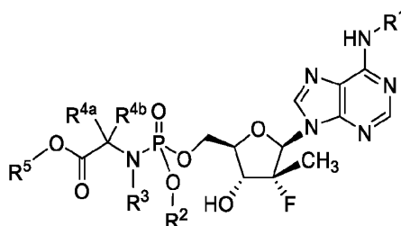
Formula II
