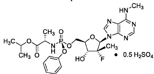
Compound 3B
