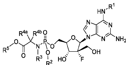
Formula IIIf
