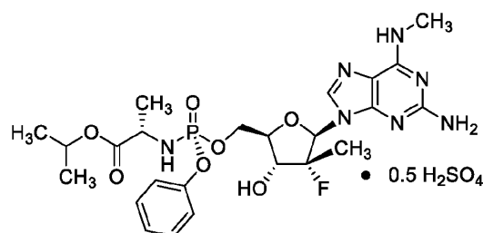
Compound 2B
