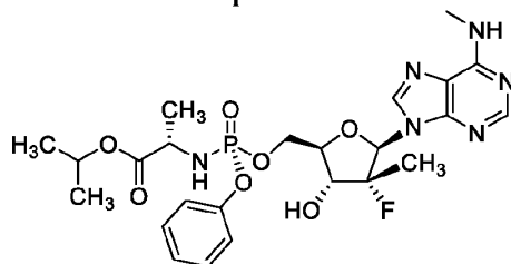
Compound 3A
