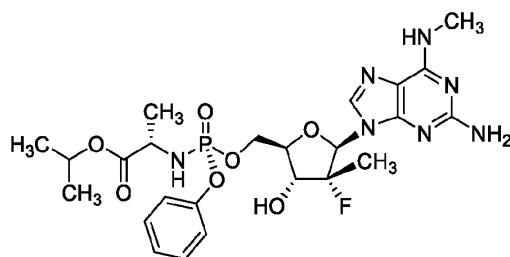
Compound 1B
