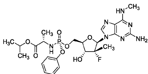
Compound 1B
