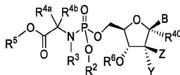
Formula VII
