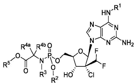
Formula IVc
