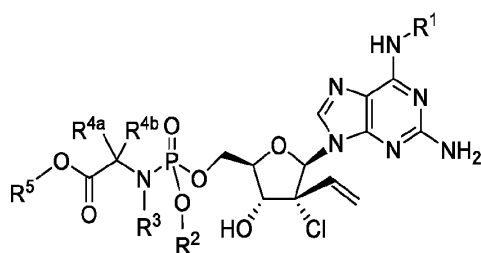
Formula IVd
