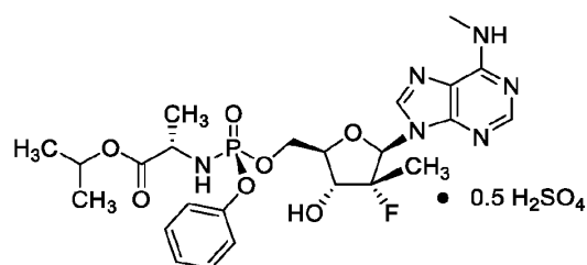
Compound 4A
