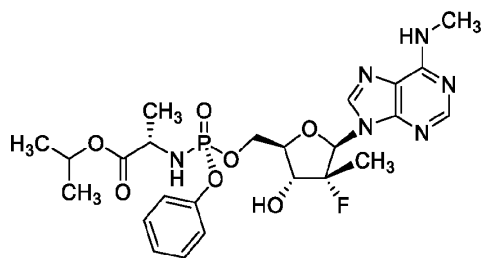
Compound 3B
