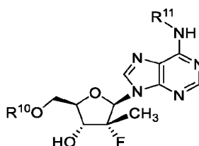
Formula X
