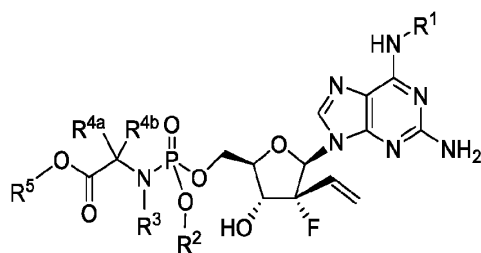
Formula IIIc
