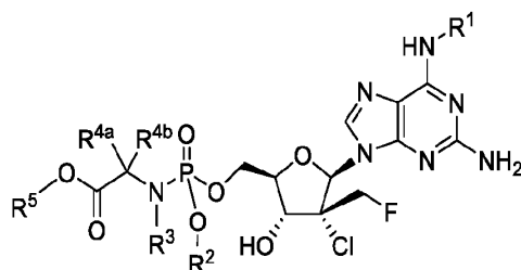
Formula IVa
