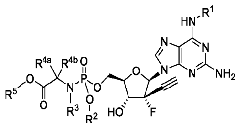
Formula IIIe
