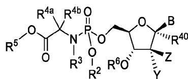
Formula VII
