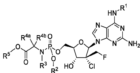
Formula IVa
