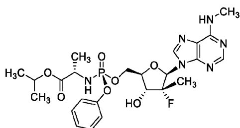
Compound 3A
