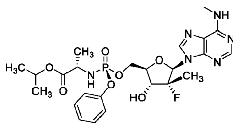
Compound 3A
