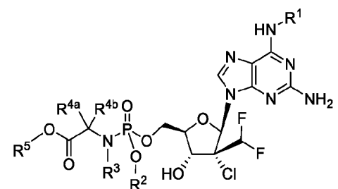
Formula IVc
