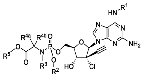
Formula IVe
