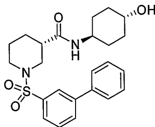
(3S)-1-(Biphenyl-3-ylsulfonyl)-N-(trans-4-hydroxycyclohexyl)piperidine-3-carboxamide
