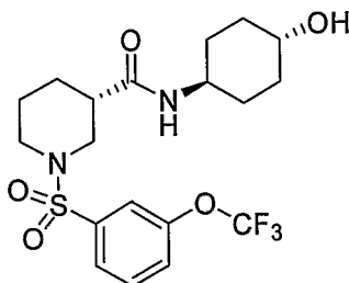
(3S)-N-(trans-4-Hydroxycyclohexyl)-1-[[3-(trifluoromethoxy)phenyl]sulfonyl]-piperidine-3-carboxamide
