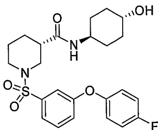
(3S)-1-[[3-(4-Fluorophenoxy)phenyl]sulfonyl]-N-(trans-4-hydroxycyclohexyl) piperidine-3-carboxamide
