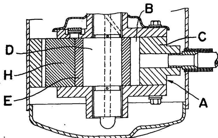
Fig. 7 PRIOR ART
