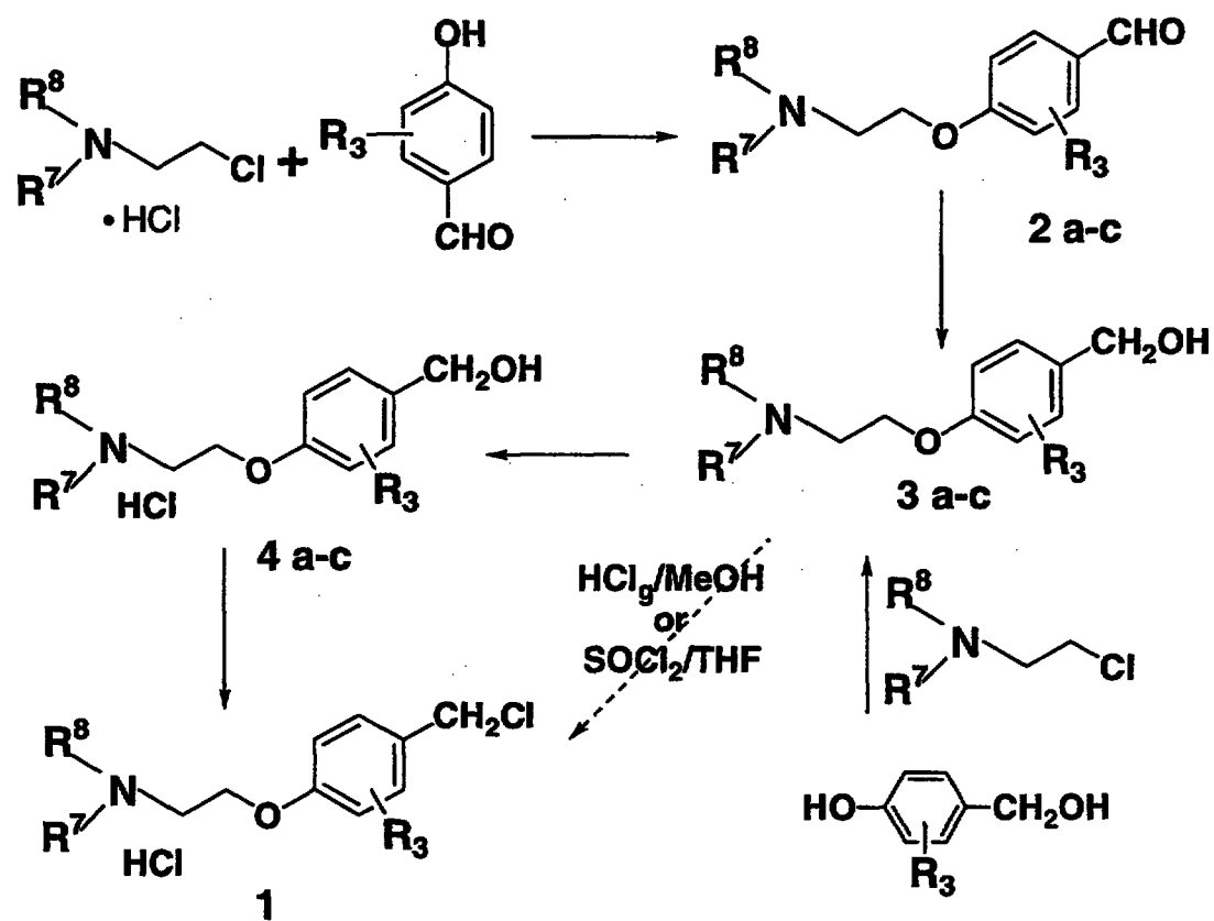
Scheme I
