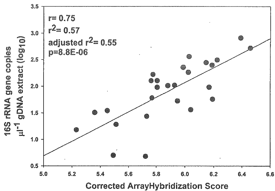
Figure S4. Comparison of real-time PCR and array monitoring of Pseudomonas oleovorans density in aerosol samples from San Antonio. Corrected Array Hybridization Score is the \ln(\text{intensity}) normalized by internal spikes as described under Normalization.
