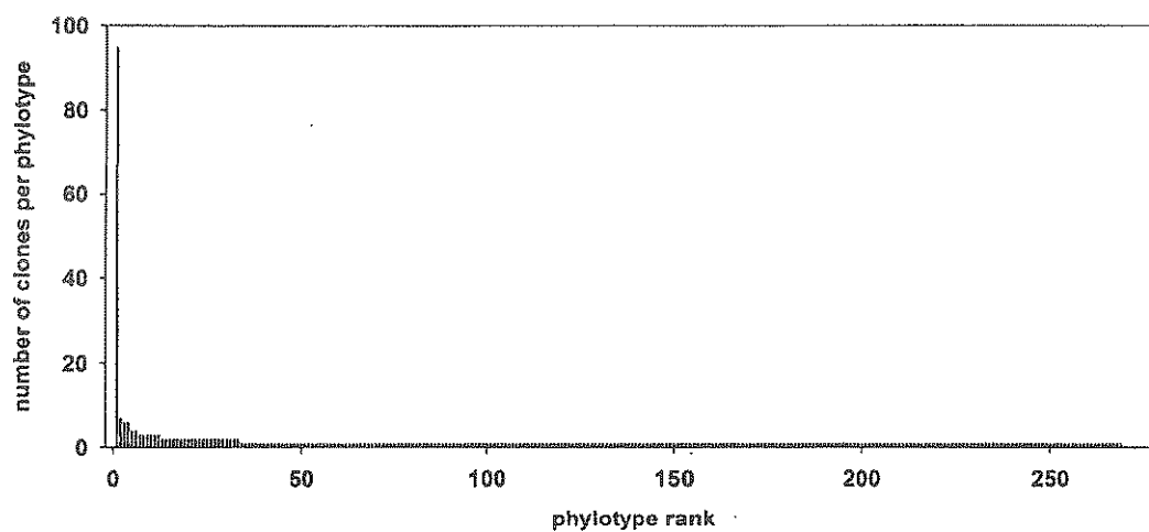
Figure S1. Rank-abundance curve of phylotypes within the urban aerosol clone library obtained from San Antonio calendar week 29. Phylotypes were determined by clustering at 99% homology using nearest neighbor joining.
