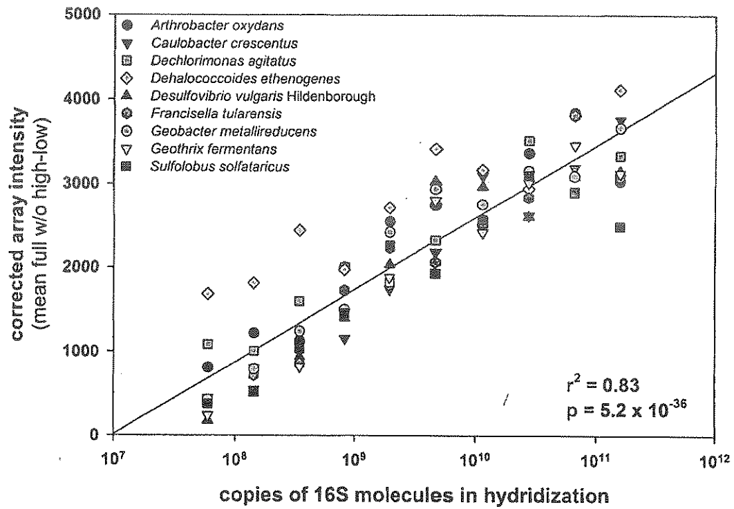
Figure S3. Latin square assessment of 16S rRNA gene sequence quantitation by microarray.
