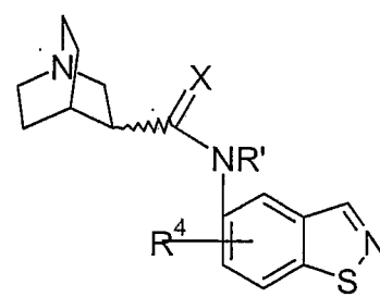
(IIIm)
