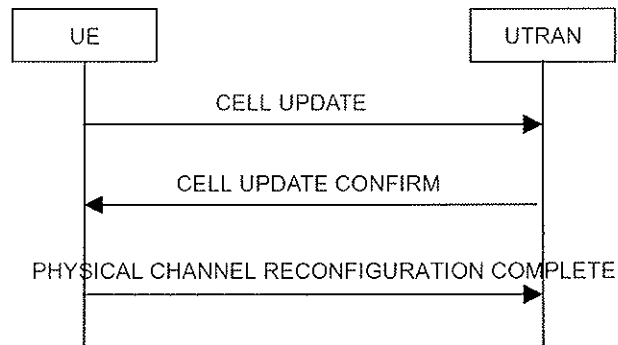
Figure 8.3.1-3: Cell update procedure with physical channel reconfiguration
