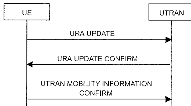
Figure 8.3.1-9: URA update procedure with update of UTRAN mobility information
