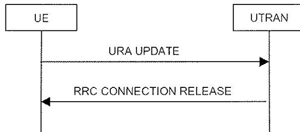
Figure 8.3.1-10: URA update procedure, failure case
