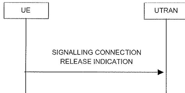
Figure 8.1.14-1: Signalling connection release indication procedure, normal case
