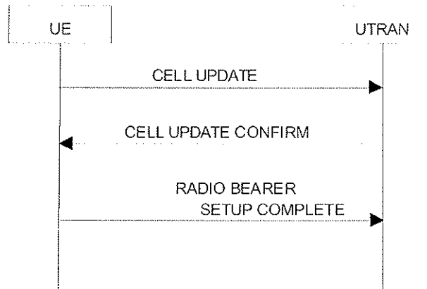
Figure 8.3.1-6a: Cell update procedure with radio bearer setup
