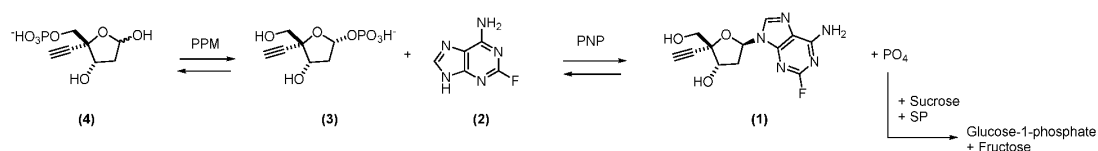
Scheme III. Overall Reaction Scheme to Produce Compound (1)
