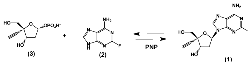
Scheme I. Reaction Catalyzed by Purine Nucleoside Phosphorylase (PNP)
