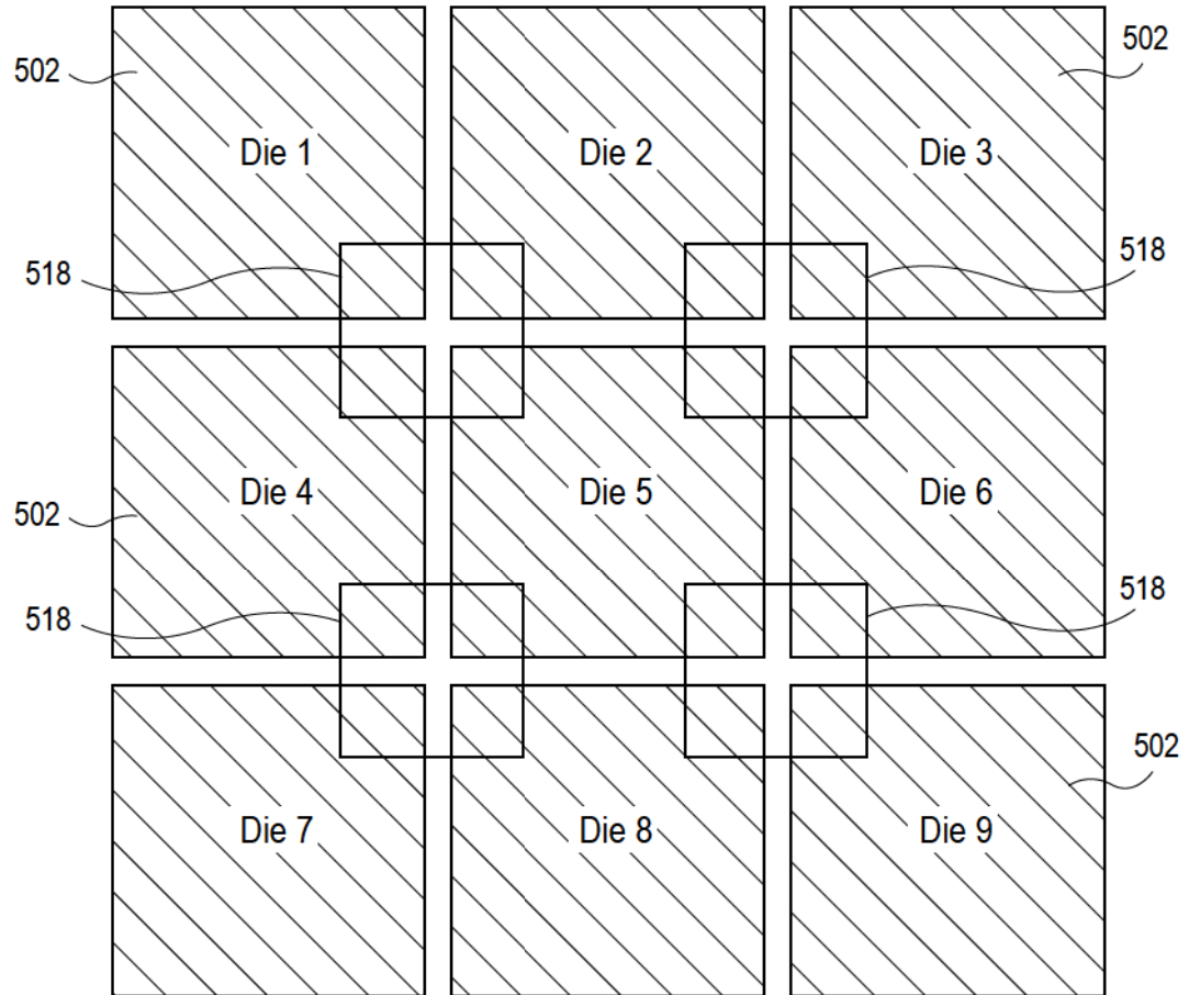
3x3 Vertical Interconnect Hub Architecture w/ 4 Hub Die
