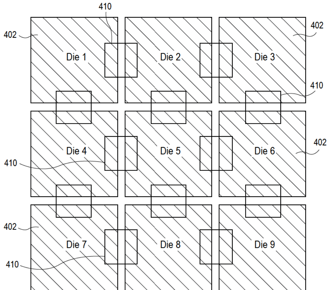
3x3 Legacy EMIB Tile Architecture w/ 12 EMIB Die
