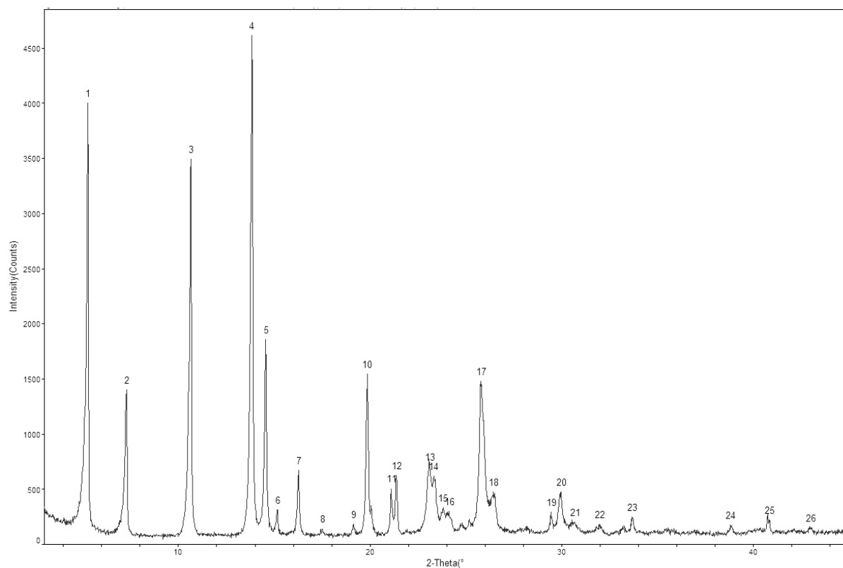
Figure 1 Powder X-ray diffractogram of Form I
