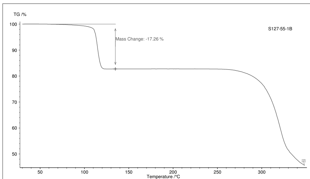
Figure 18 Thermogravimetric (TG) curve of Form VIII
