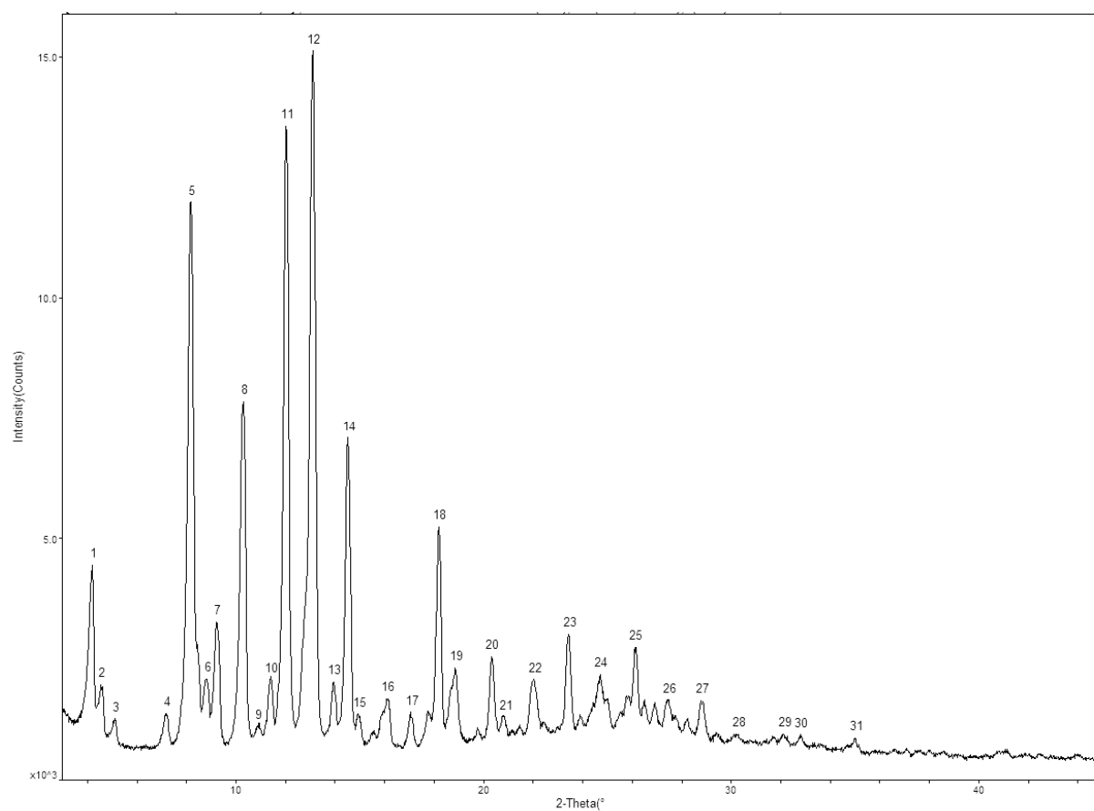
Figure 4 Powder X-ray diffractogram of Form II
