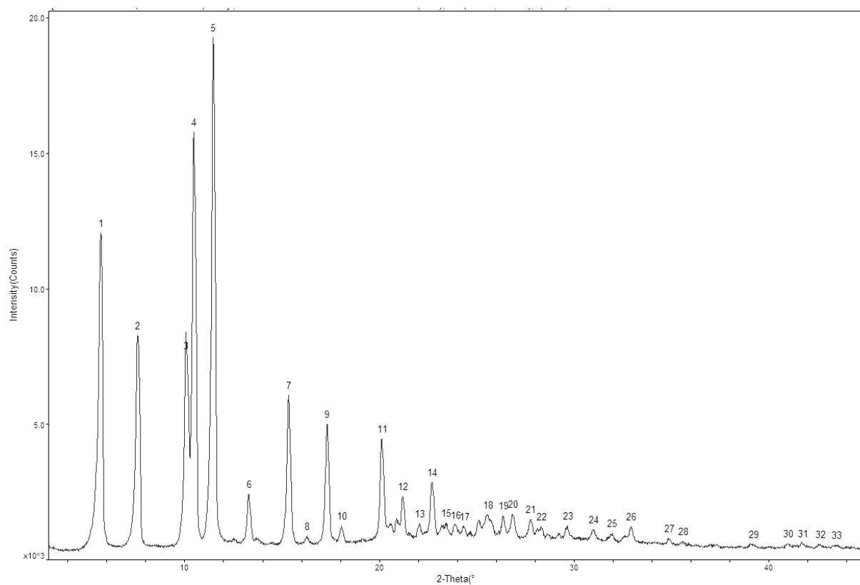
Figure 10 Powder X-ray diffractogram of Form IV
