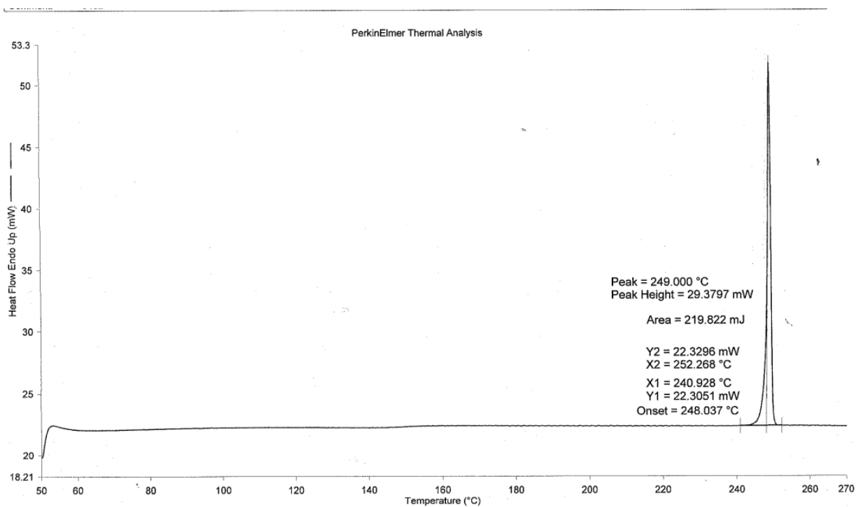
Figure 8 Differential scanning calorimeter (DSC) thermogram of Form III
