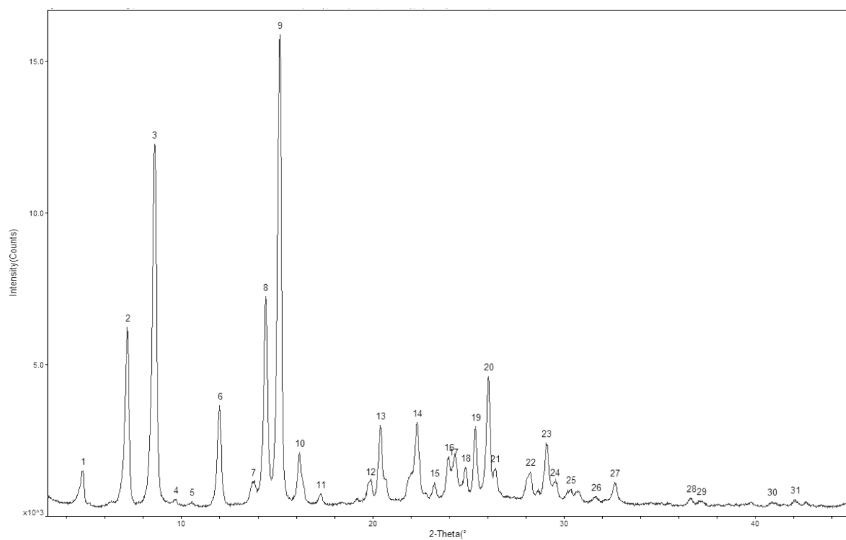
Figure 7 Powder X-ray diffractogram of Form III
