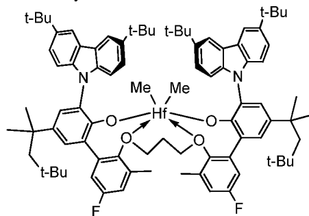
Procatalyst 3
