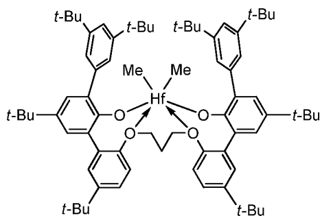
Procatalyst 2
