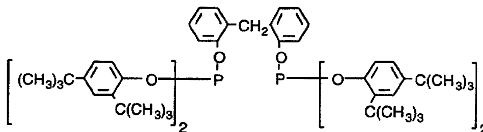
Ligand U
