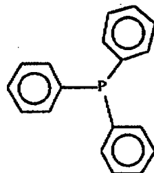
Triphenylphosphine, (TPP)
