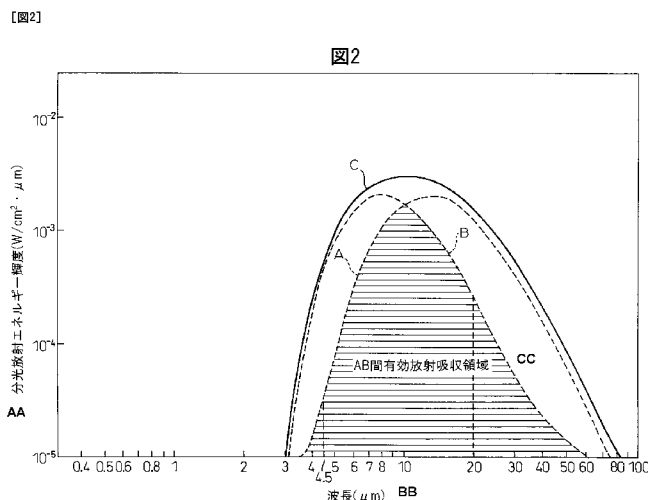
FIG. 2: AA Spectral emission energy luminance ( \text{W}/\text{cm}^2 \cdot \mu\text{m} ) BB Wavelength ( \mu\text{m} ) CC Effective radiation absorption region between (A) and (B)
