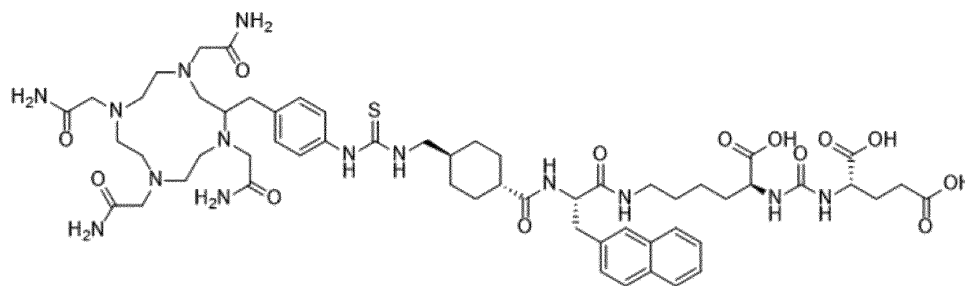
p-SCN-Bn-TCMC-PSMA ligand 1
