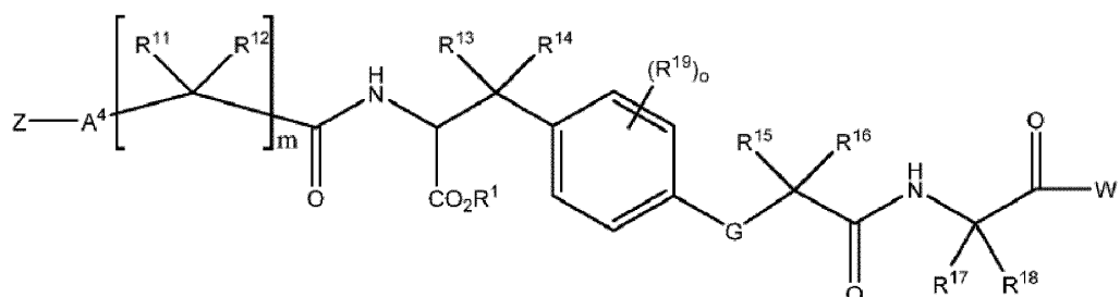
Formula I
