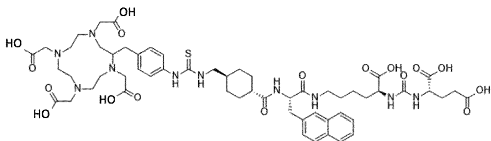
p-SCN-Bn-DOTA-PSMA ligand 2
