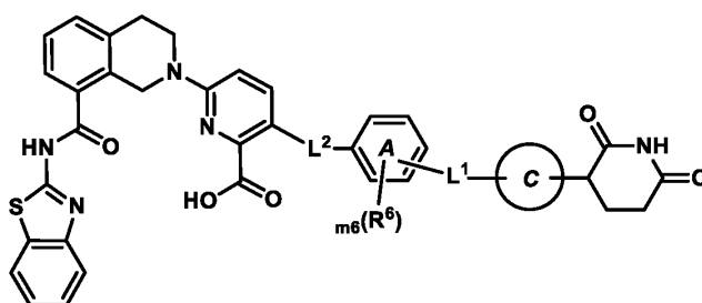
Formula (I-a)
