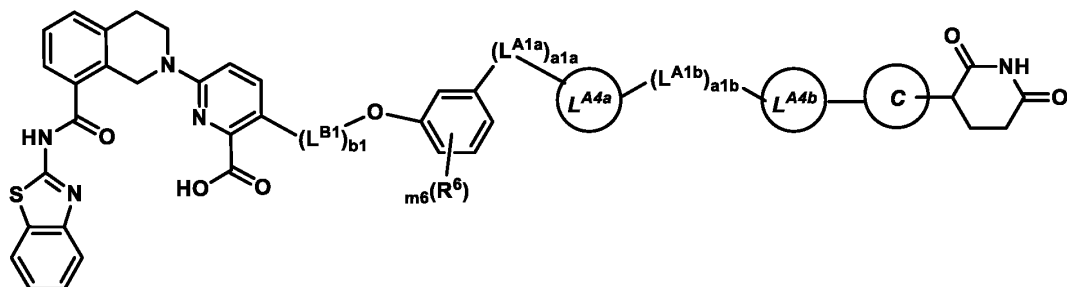
Formula (I-b1)
