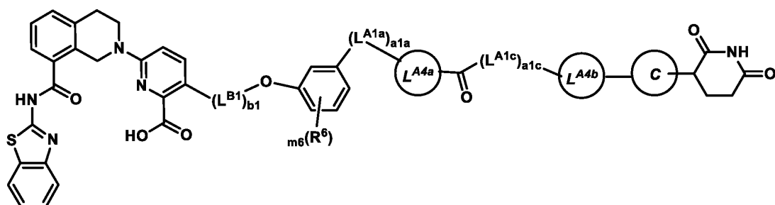
Formula (I-b3)
