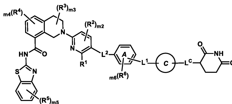
Formula (I)
