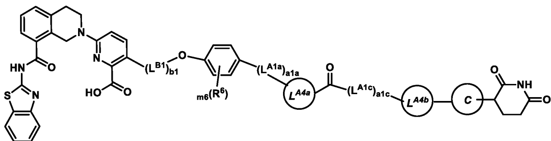
Formula (I-b4)
