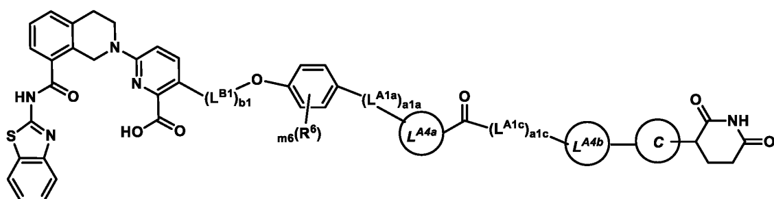
Formula (I-b4)
