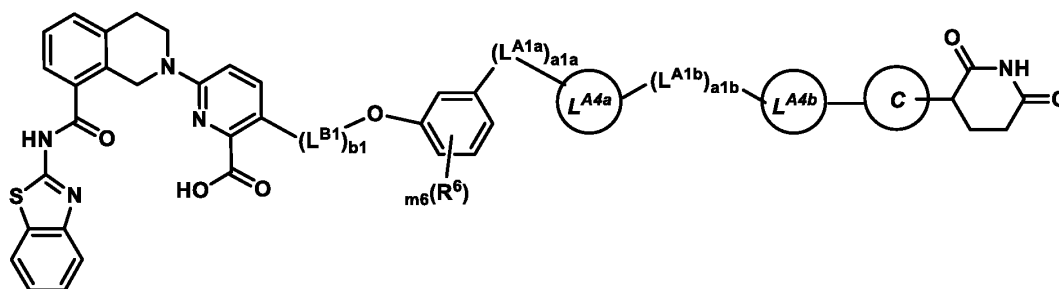
Formula (I-b1)
