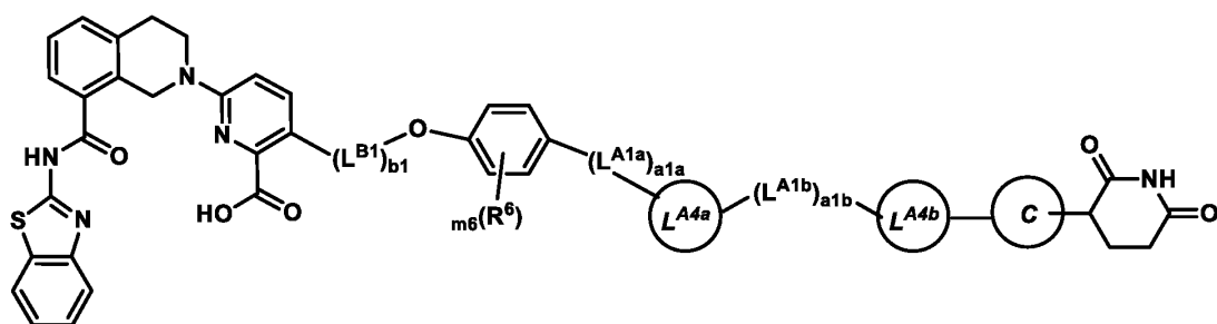
Formula (I-b2)
