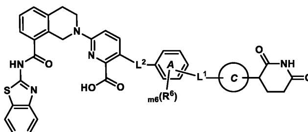
Formula (I-a)
