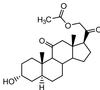
Formula (VI)
