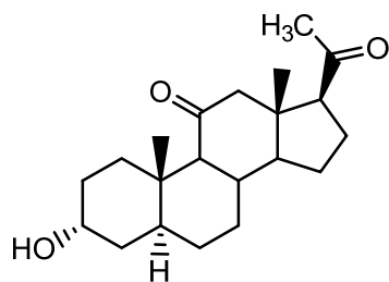
Formula (Ia)
