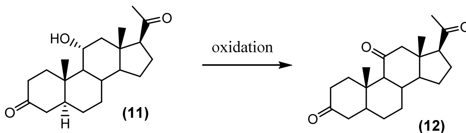
Scheme 5: Oxidation of 11α-hydroxy-3,20-diketo-5α-H-pregnane (11) to 3,11,20-triketo-5α-H-pregnane (12)
