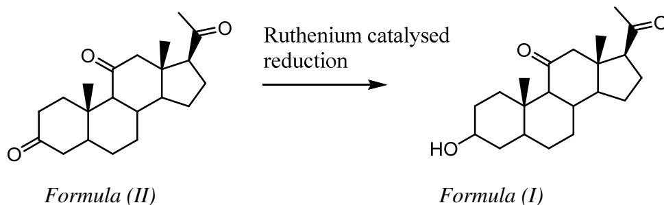
Scheme 2: Ruthenium catalyzed reduction of compounds of Formula (II)
