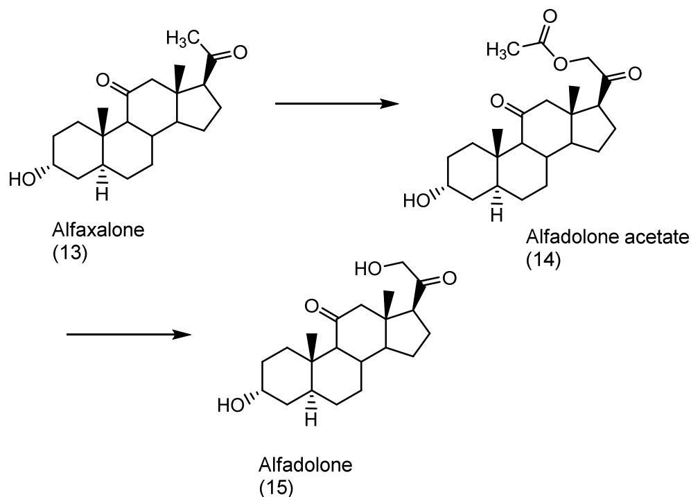
Scheme 6: Preparation of alfadolone and alfadolone acetate from alfaxalone
