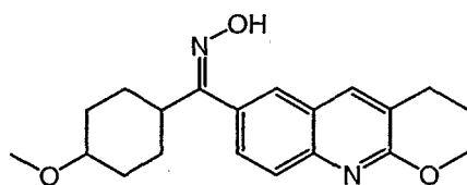
[1α(A),4α] (compound 51)
