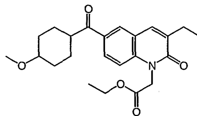
(trans) (compound 45)
