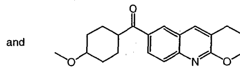
TRANS
