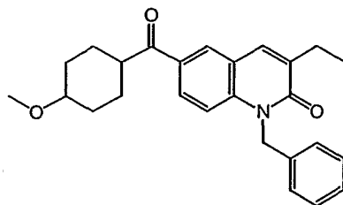
cis (compound 46)
