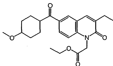
cis (compound 44)
