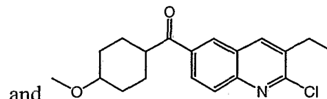
trans (compound 5)
