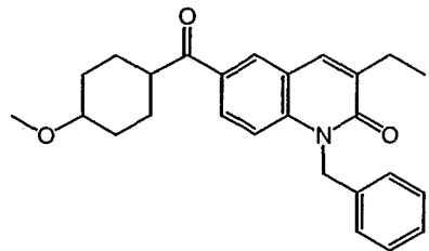
(trans) (compound 47)
