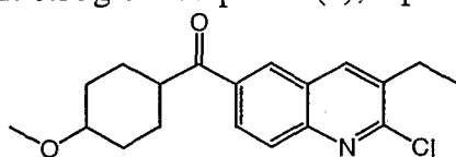
cis (compound 4)
