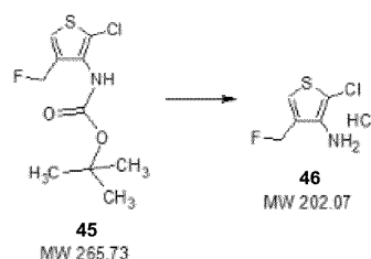
2-chloro-4-(fluoromethyl)thiophen-3-amine hydrochloride
