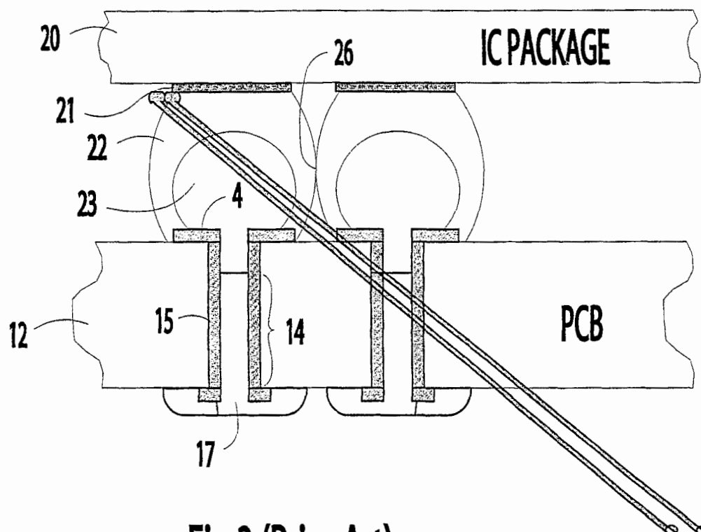
Fig.3 (Prior Art)
