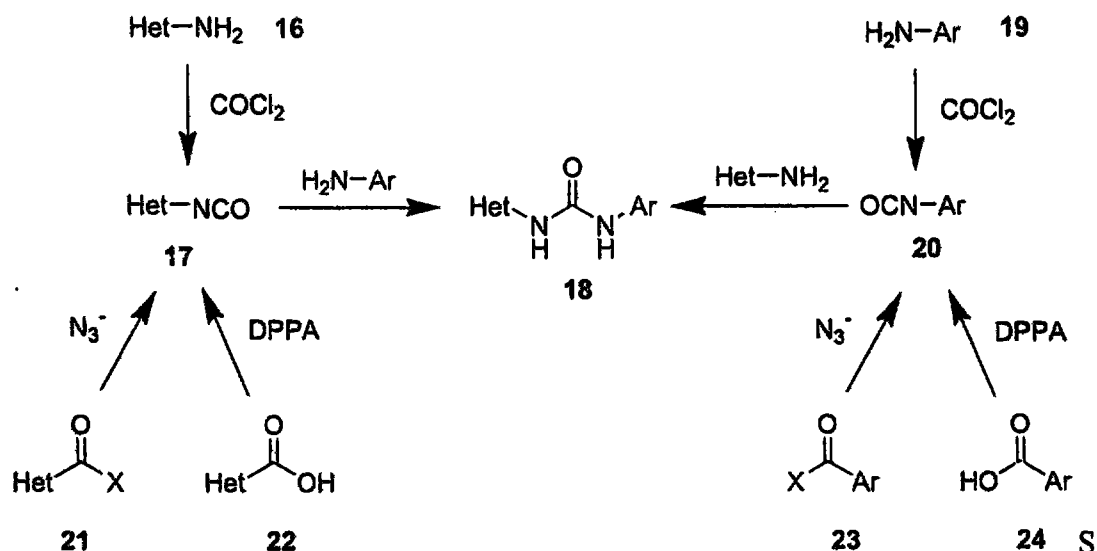
Scheme IV Selected Methods of Urea Formation (Het = heterocycle)
