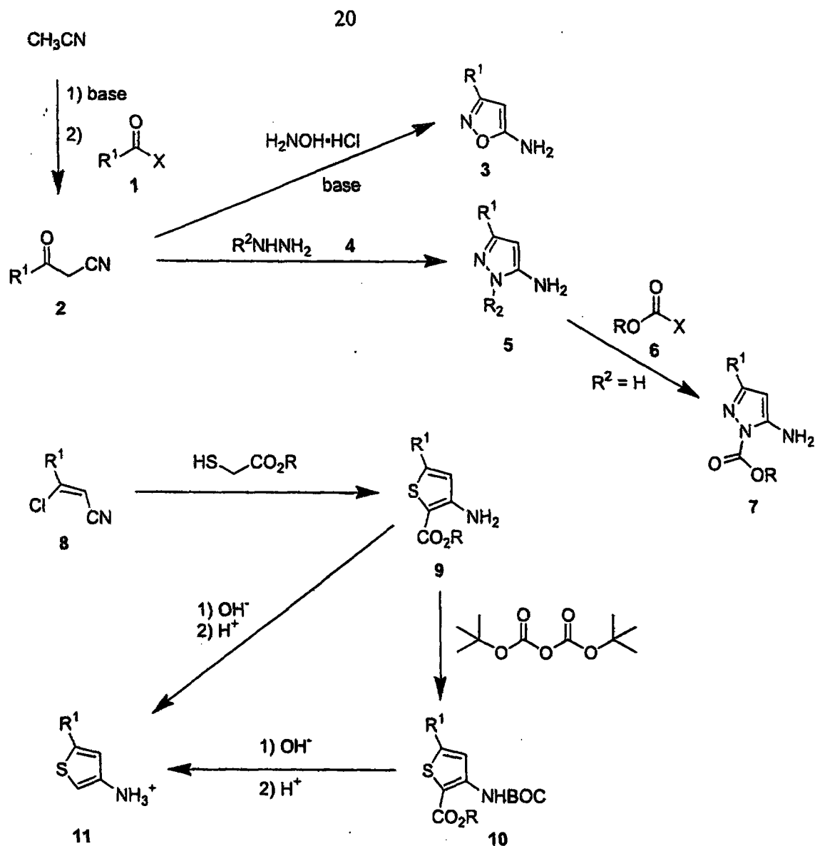
Scheme I. Selected General Methods for Heterocyclic Amine Synthesis
