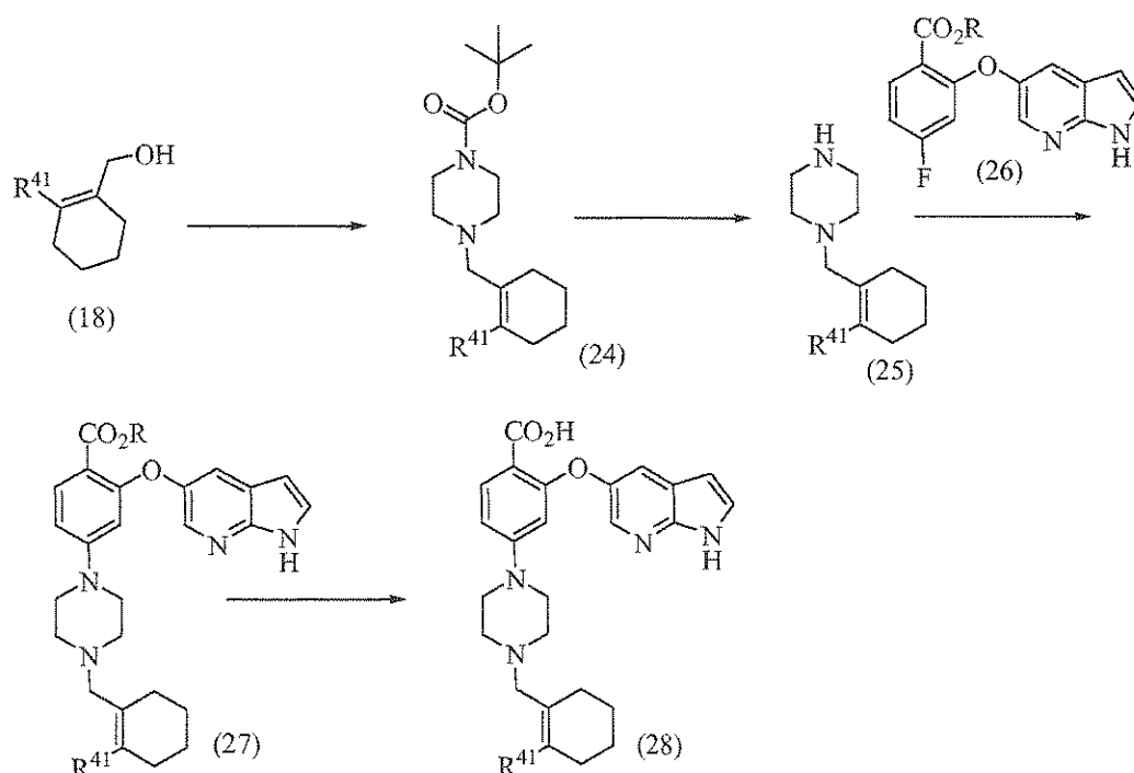
SCHEME 6
