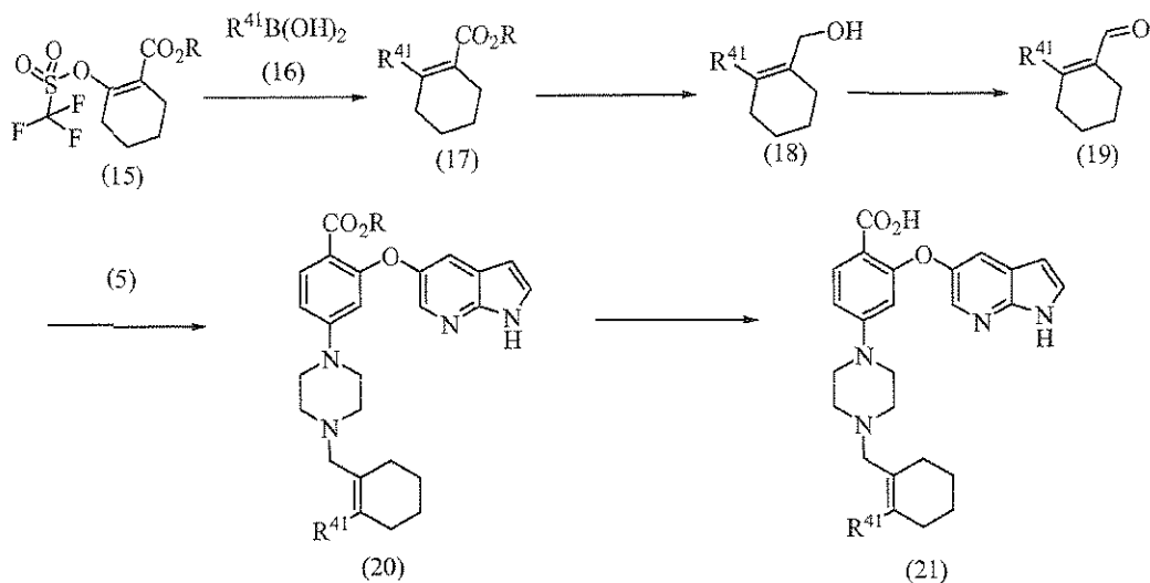
SCHEME 4
