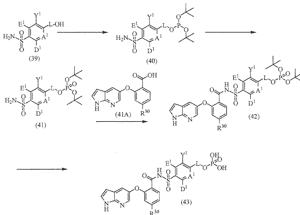
SCHEME 12
