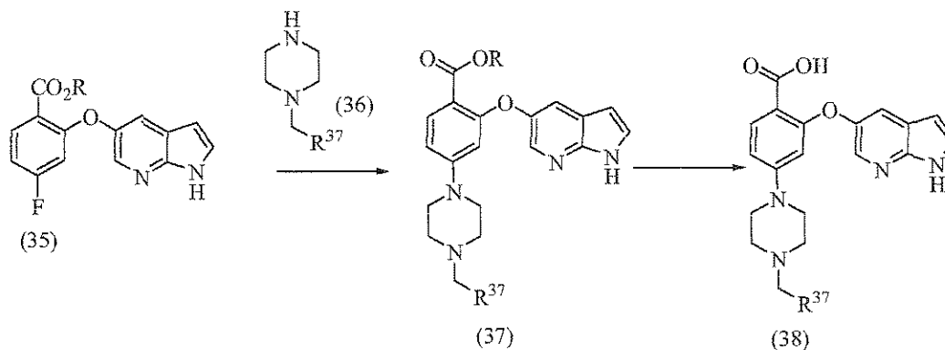
15 SCHEME 9
