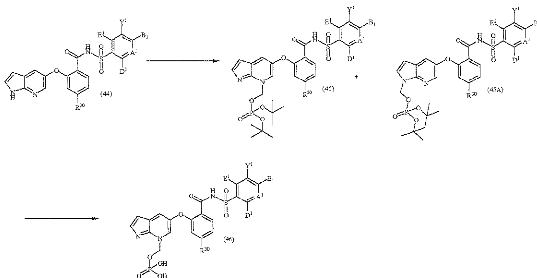
SCHEME 13
