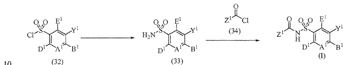
SCHEME 8
