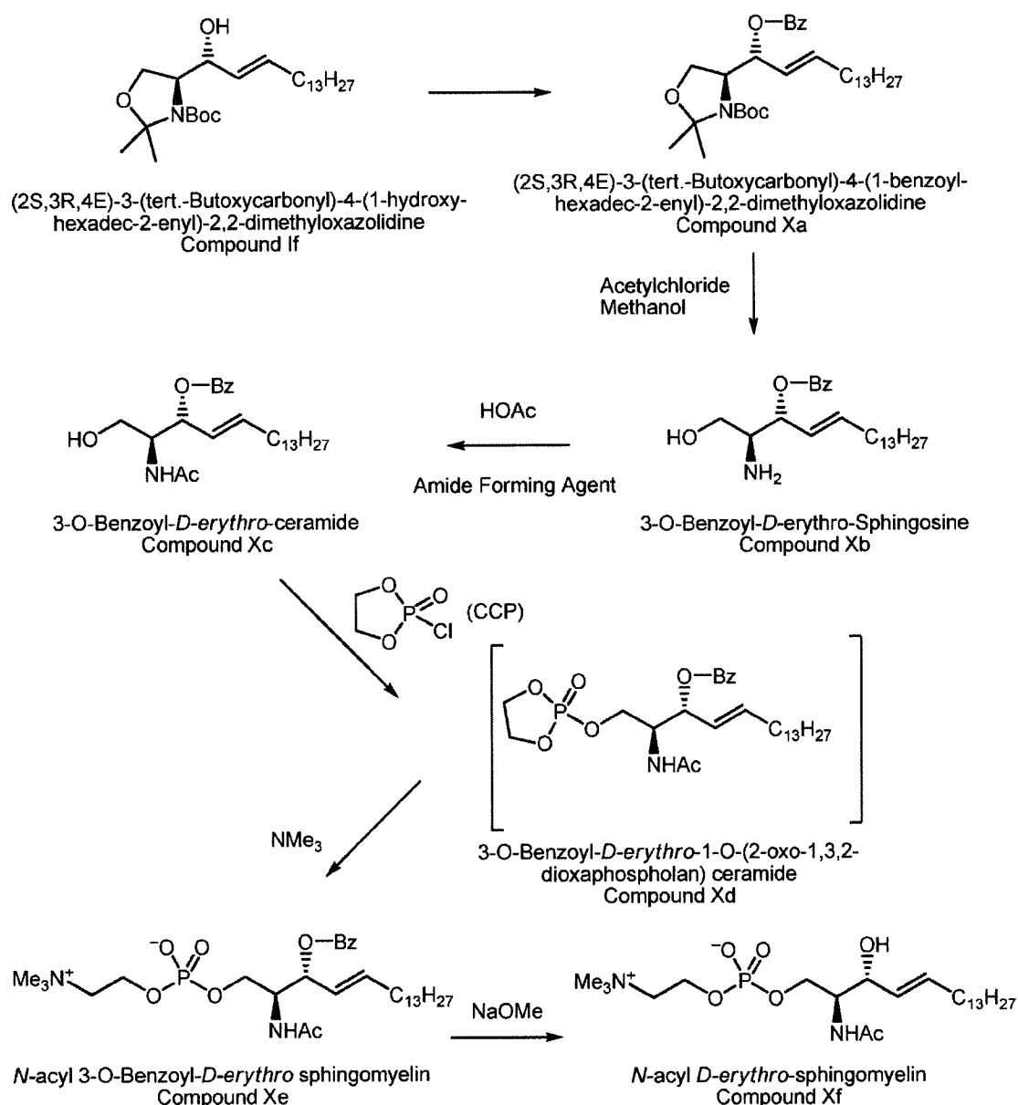
Scheme X
