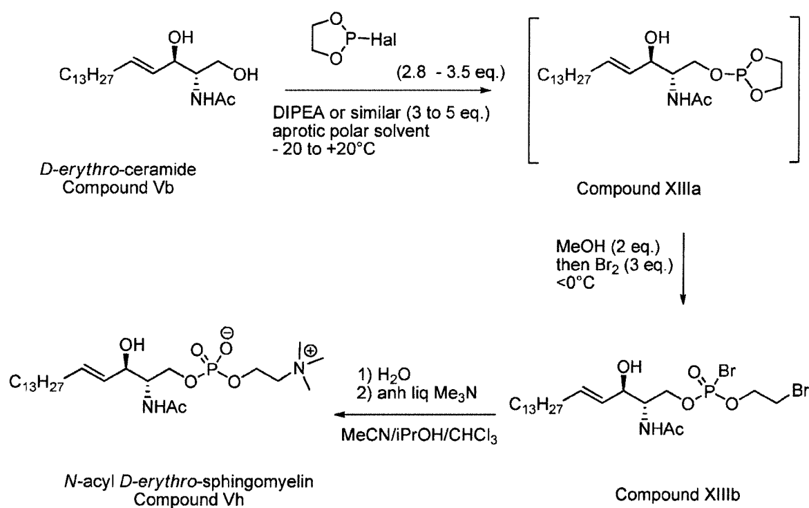
Scheme XIII
