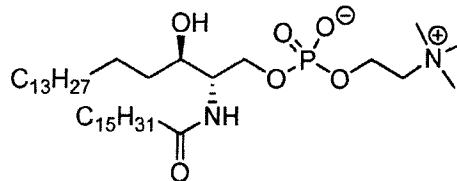
Compound D
