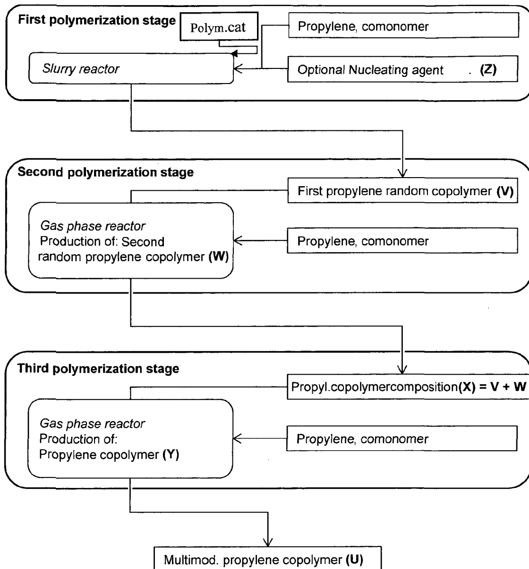
Scheme 1.
