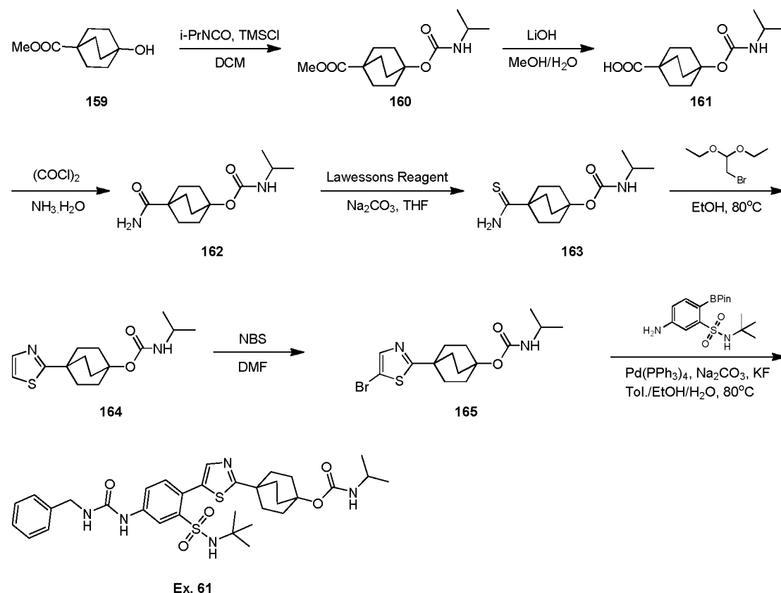
Scheme 22:
