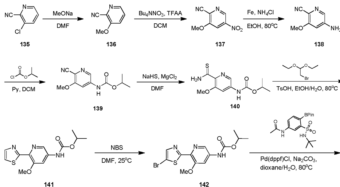
Scheme 18:
