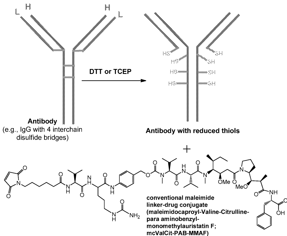
Scheme C ADCs conjugated with mcValCit-PAB-MMAF
