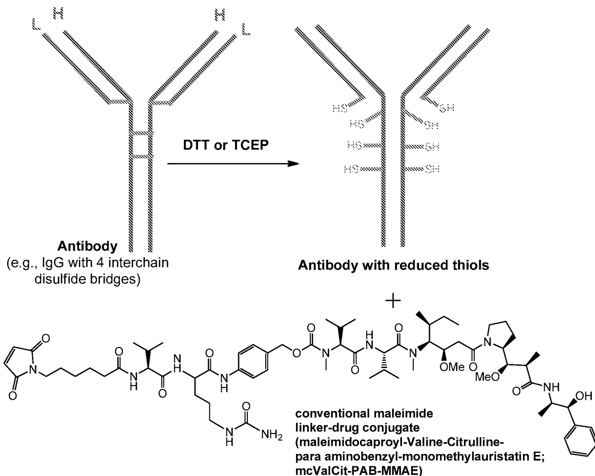
Scheme D ADCs conjugated with mcValCit-PAB-MMAE
