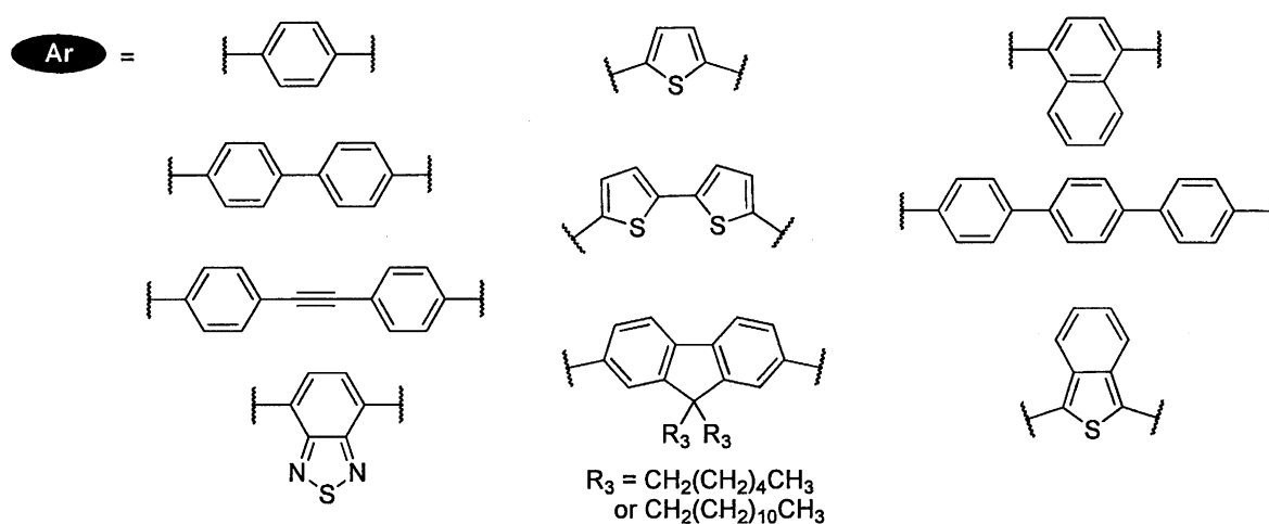
Scheme 2: Optional connectivity of the group \text{Ar} in Formula (I) of the present disclosure
