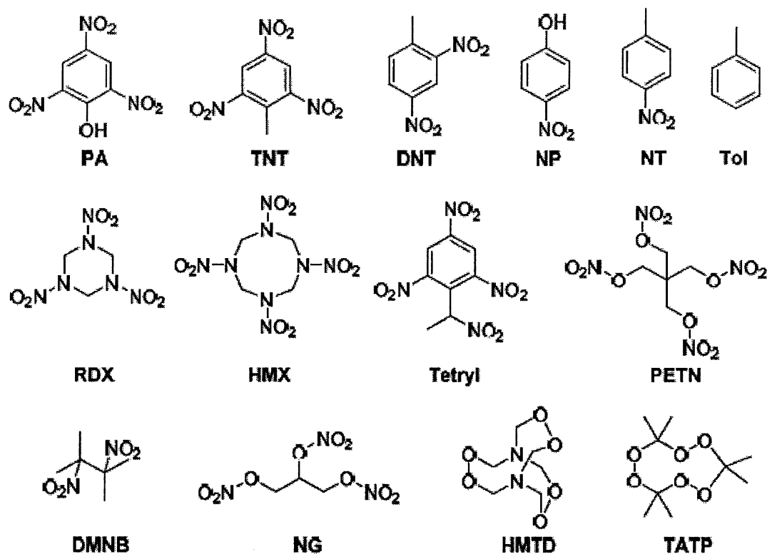
Scheme 1: Structural illustration of explosives and examples, including PA (picric acid), TNT (2,4,6-trinitrotoluene), DNT (2,4-dinitrotoluene), NT (4-nitrotoluene), Tol (toluene), RDX (1,3,5-Trinitro-1,3,5-triazacyclohexane), HMX (Octahydro-1,3,5,7-tetranitro-1,3,5,7-tetrazocine), Tetryl (2,4,6-Trinitrophenylmethylnitramine), PETN (Pentaerythritol tetranitrate), DMNB (2,3-Dimethyl-2,3-dinitrobutane), NG (Nitroglycerin), HMTD (Hexamethylene triperoxide diamine) and TATP (Triacetone triperoxide).
