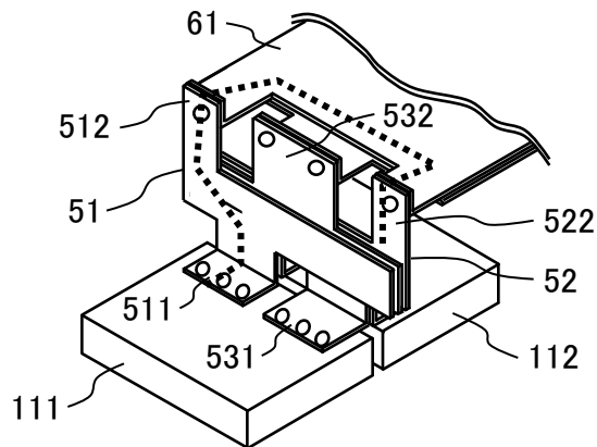
(B) EXAMPLE OF FIGS. 12 AND 14 OF PATENT DOCUMENT 1
