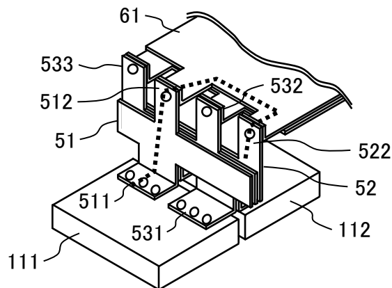
(C) EXAMPLE OF FIGS. 23 AND 24 OF PATENT DOCUMENT 1
