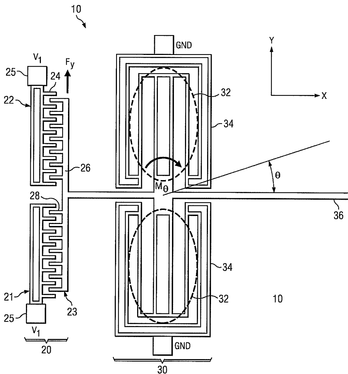
FIG. 1 (PRIOR ART)
