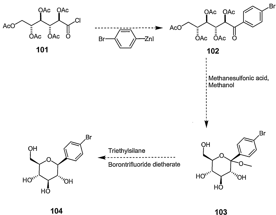
Scheme 7
