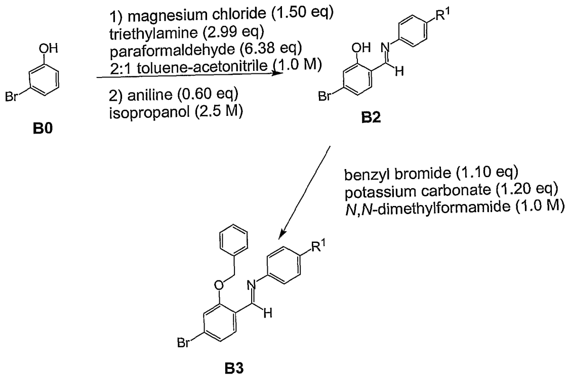
Scheme 2
