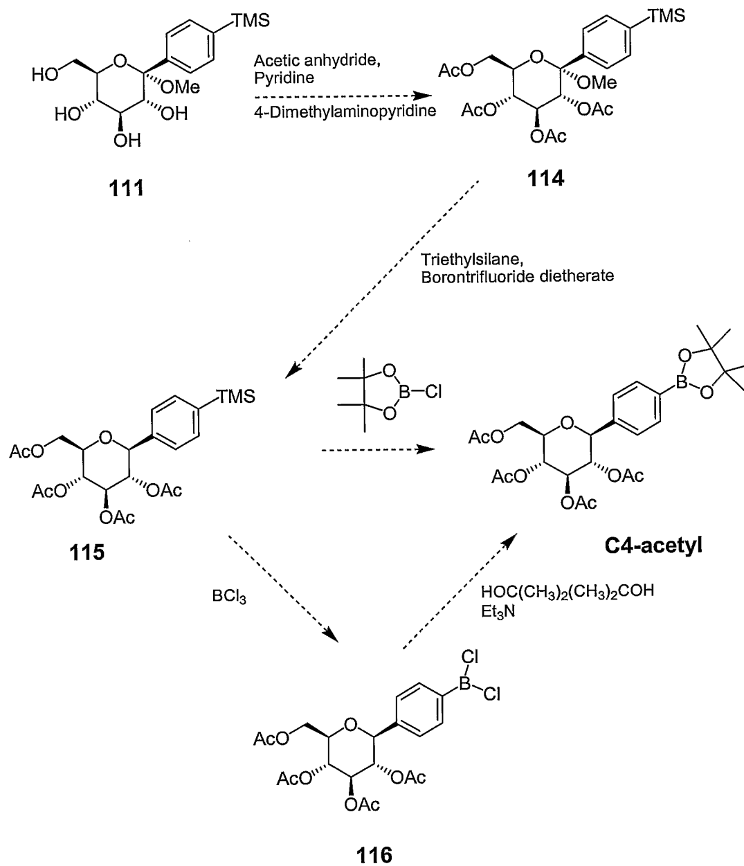
Scheme 9
