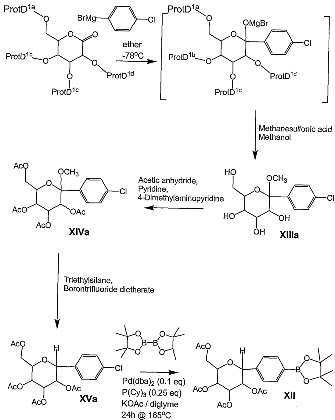
Scheme 6
