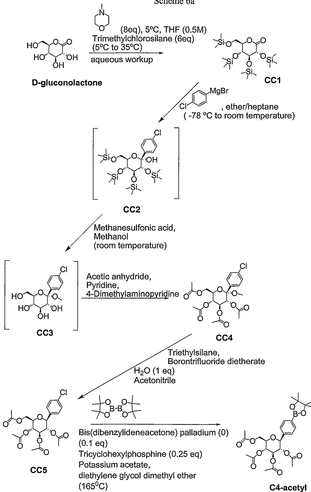
Scheme 6a
