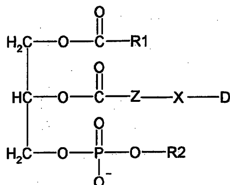
Formula I
