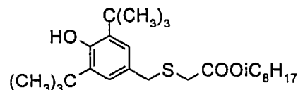
Phenol X
