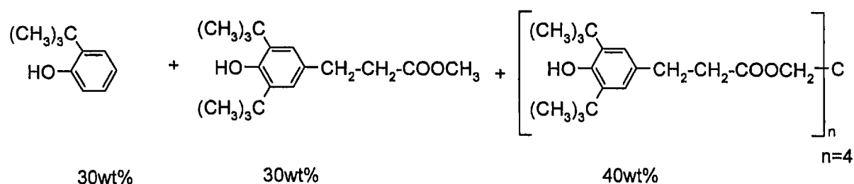
Phenol U
