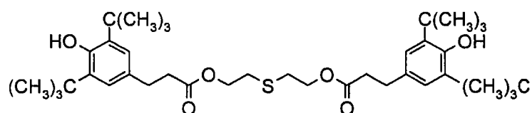
Phenol W
