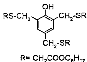
Phenol V
