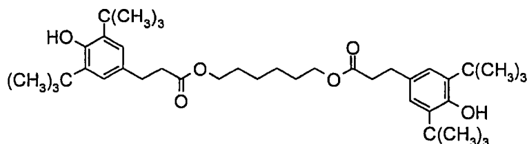
Phenol W
