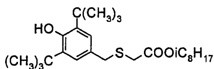
Phenol S
