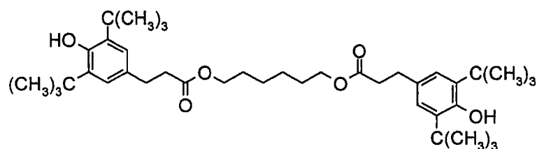
Phenol S
