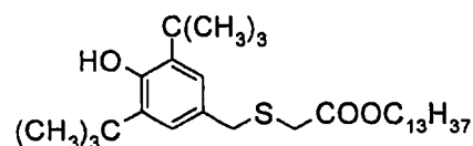
Phenol U
