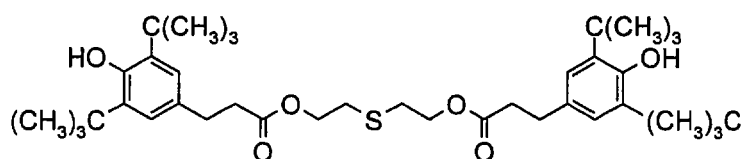
Phenol W
