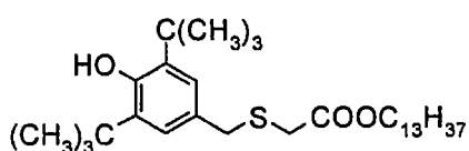
Phenol X
