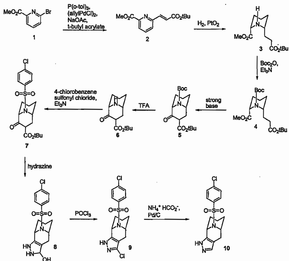
Scheme 2
