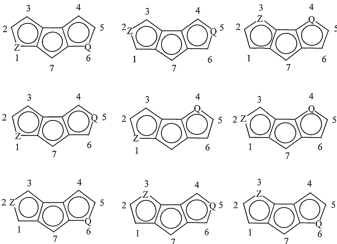
heterofluorenyl ligands
