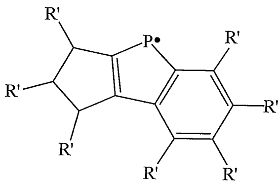
1,2,3,4-tetrahydro-cyclopenta[b]phosphindol-4-yl
