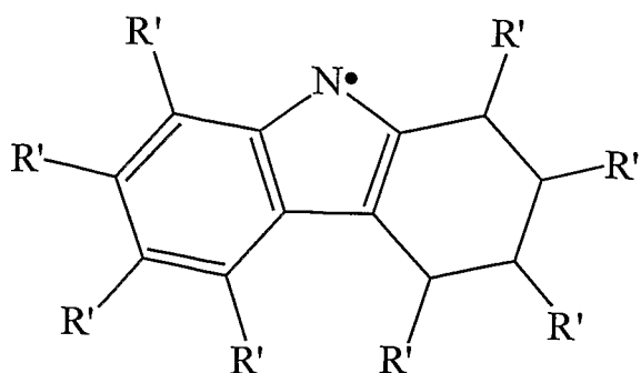
1,2,3,4-tetrahydro-carbazol-9-yl
