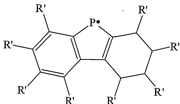
1,2,3,4-tetrahydro-dibenzophosphol-5-yl
