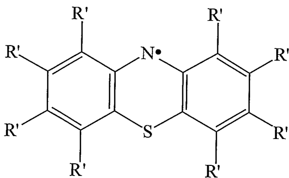
phenothiazin-10-yl
