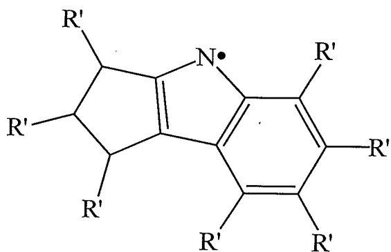
1,2,3,4-tetrahydro-cyclopenta[b]indol-4-yl
