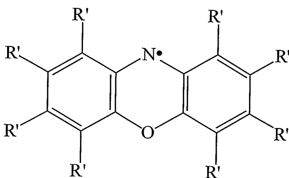
phenoxazin-10-yl
