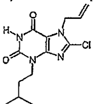
a) 8-chloro-3-(3-methylbutyl)-7-(2-propen-1-yl)-3,7-dihydro-1H-purine-2,6-dione
