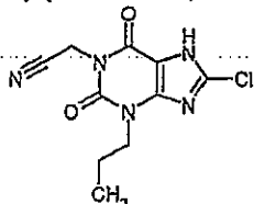
b) (8-chloro-2,6-dioxo-3-propyl-2,3,6,7-tetrahydro-1H-purin-1-yl)acetonitrile
