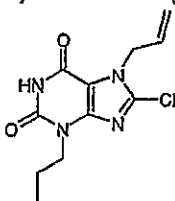
a) 8-chloro-7-(2-propen-1-yl)-3-propyl-3,7-dihydro-1H-purine-2,6-dione
