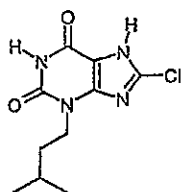
a) 8-chloro-3-(3-methylbutyl)-7-(2-propen-1-yl)-3,7-dihydro-1H-purine-2,6-dione
